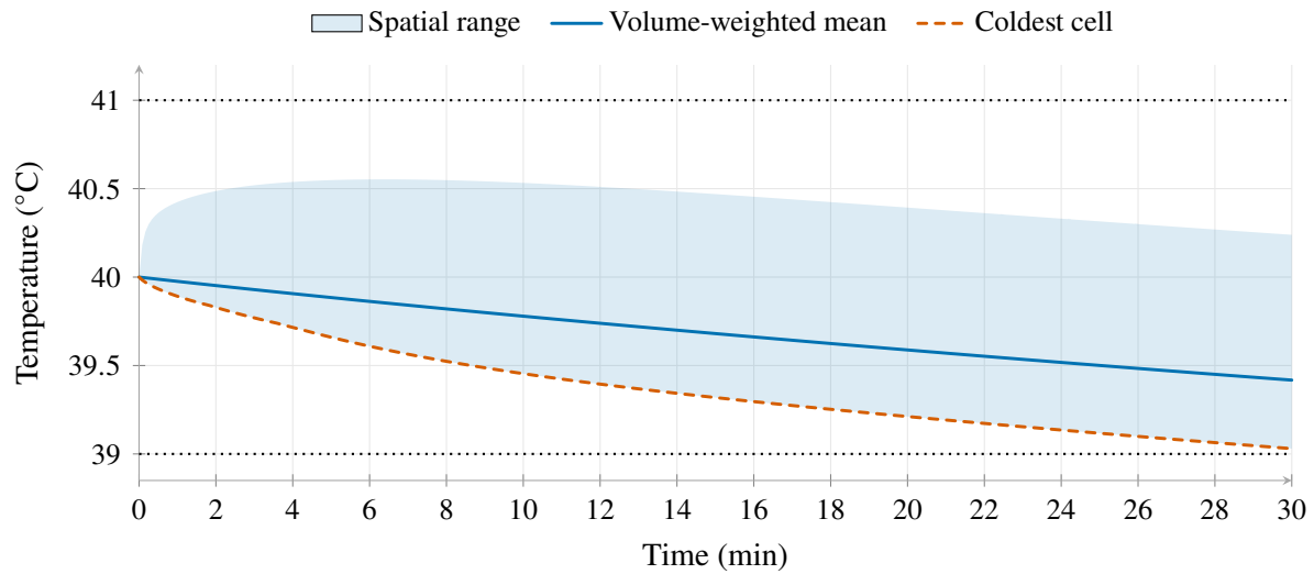
Figure 3. Matrix-exponential cell temperatures under the selected policy. The shaded range includes all cells; the mean alone would hide cold and hot locations.
