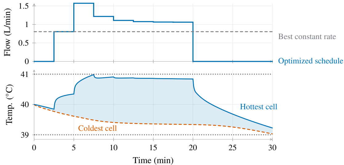
Figure 4. Best 12-segment schedule against the best constant rate (top) and the range of cell temperatures (bottom); dotted lines mark the limits.
