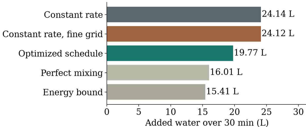
Figure 4. Water-use comparison under the same lower limit. The energy bound is conditional on the network assumptions; the feasible spatial result remains above it.
