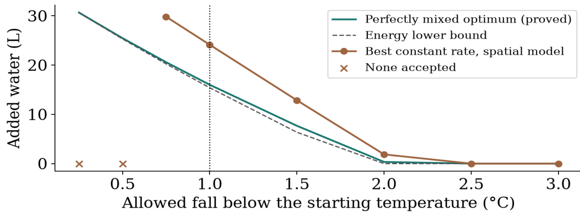
Figure 7. Added water against the allowed temperature fall. The mixed optimum and energy bound are closed forms; markers on the brown curve are searched constant-rate policies, and the dotted line is the baseline.
