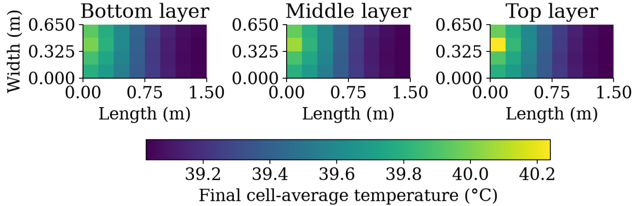
Figure 4. Final temperatures in the three horizontal cell layers. All layers use one color scale; the top layer contains the prescribed inlet-to-overflow stream. Geometry is in metres, and values are cell averages.
