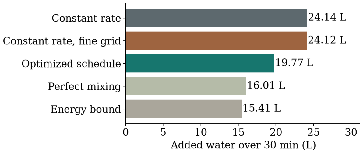
Figure 8. Water-use comparison under the same lower limit. The energy bound is conditional on the network assumptions; the feasible spatial result remains above it.
