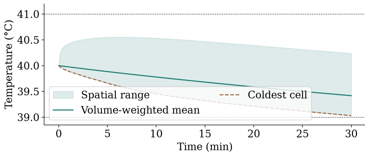
Figure 5. Matrix-exponential cell temperatures under the selected policy. The shaded range includes all cells; the mean alone would hide cold and hot locations.
