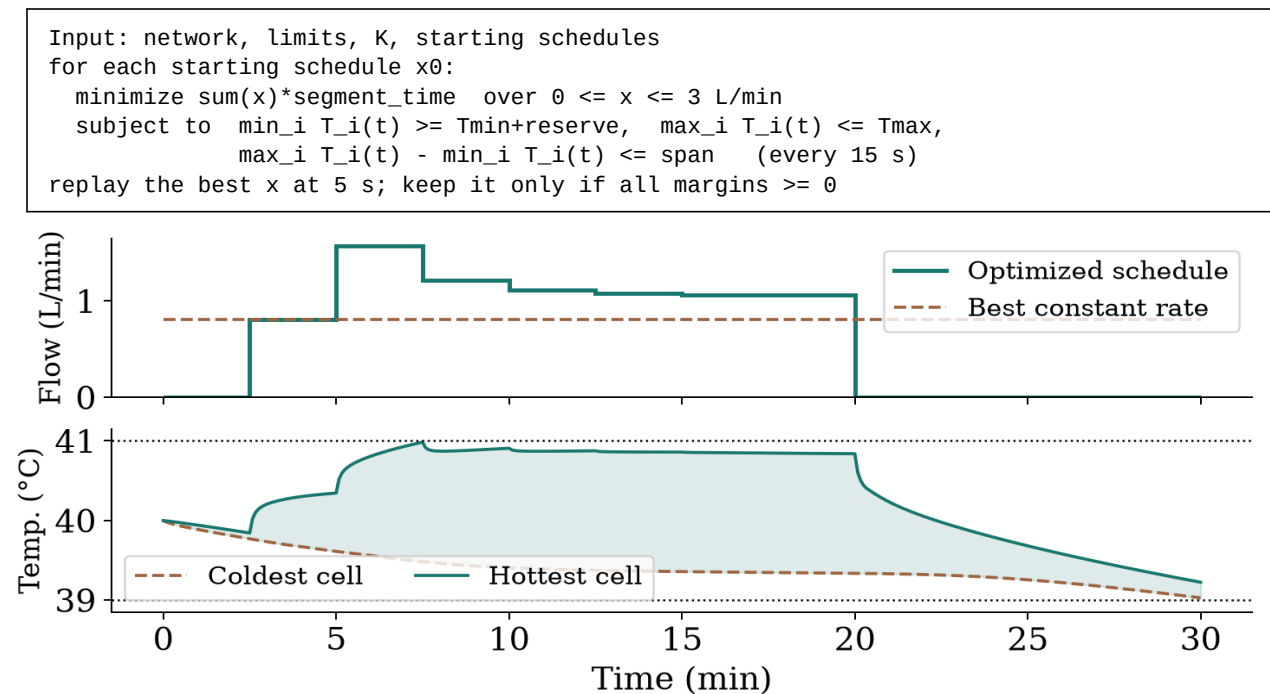
Figure 6. Best 12-segment schedule against the best constant rate (top) and the range of cell temperatures (bottom); dotted lines mark the limits.
