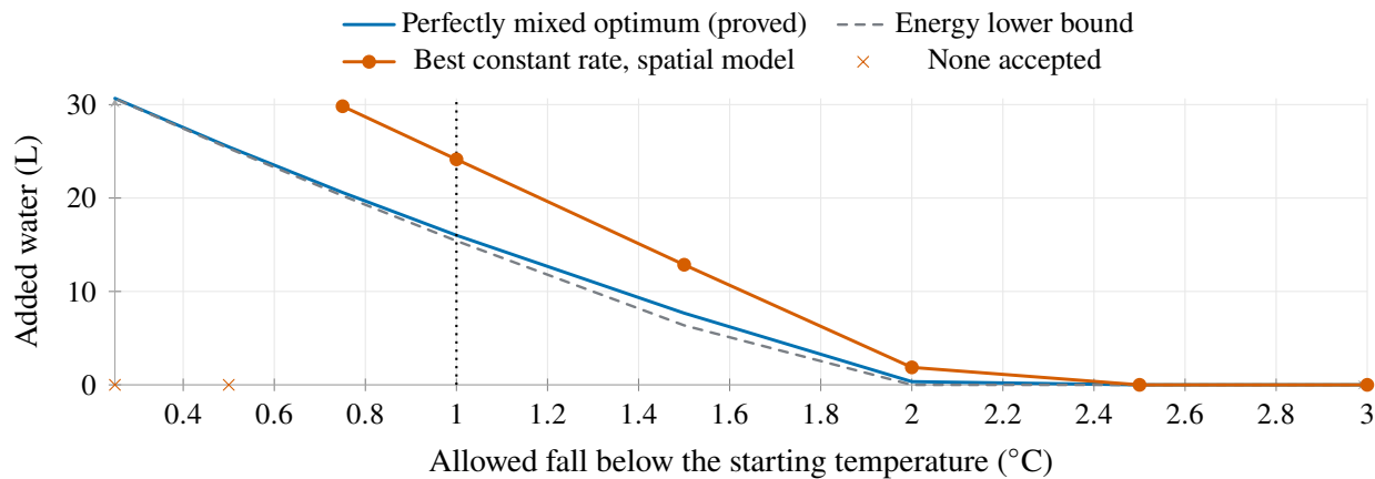
Figure 5. Added water against the allowed temperature fall. The mixed optimum and energy bound are closed forms; markers on the brown curve are searched constant-rate policies, and the dotted line is the baseline.
