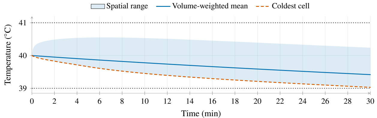
Figure 3. Matrix-exponential cell temperatures under the selected policy. The shaded range includes all cells; the mean alone would hide cold and hot locations.
