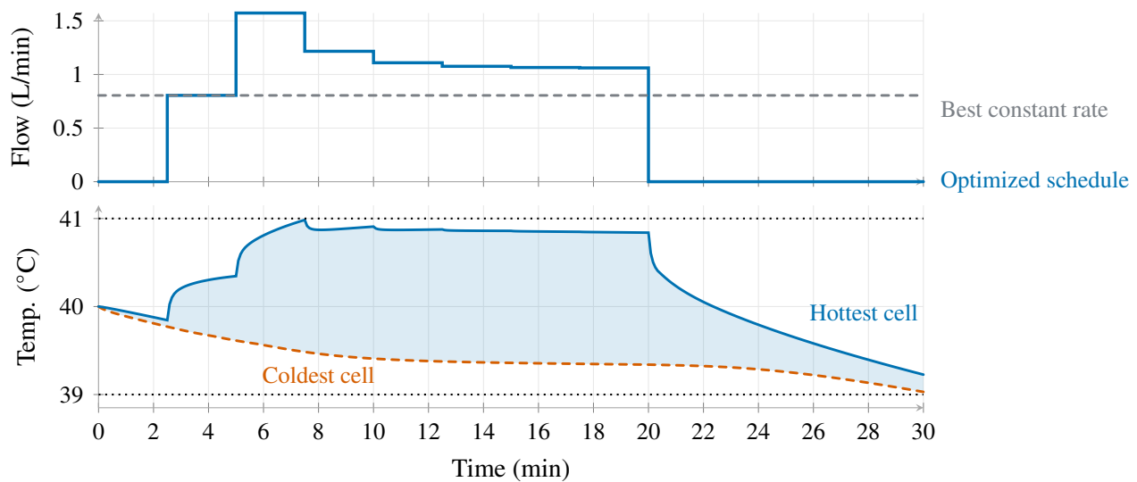
Figure 4. Best 12-segment schedule against the best constant rate (top) and the range of cell temperatures (bottom); dotted lines mark the limits.
