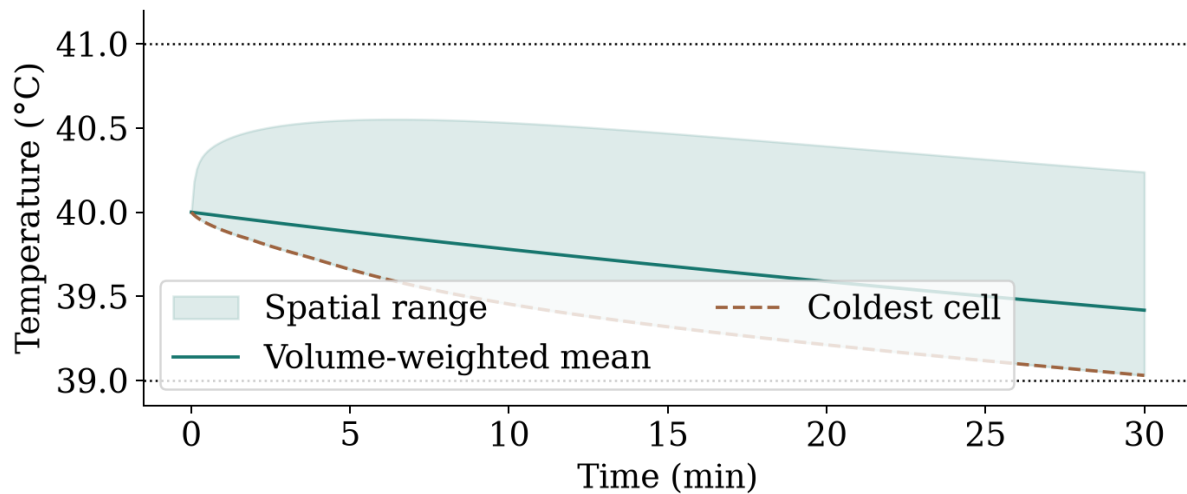
Figure 2. Matrix-exponential cell temperatures under the selected policy. The shaded range includes all cells; the mean alone would hide cold and hot locations.
