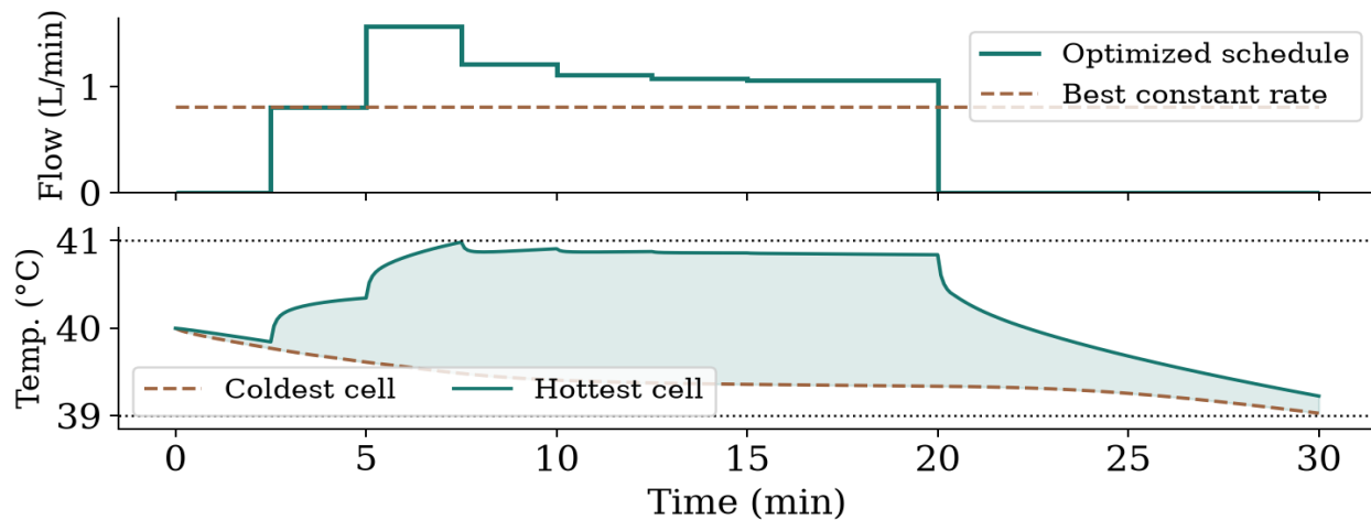
Figure 3. Best 12-segment schedule against the best constant rate (top) and the range of cell temperatures (bottom); dotted lines mark the limits.
