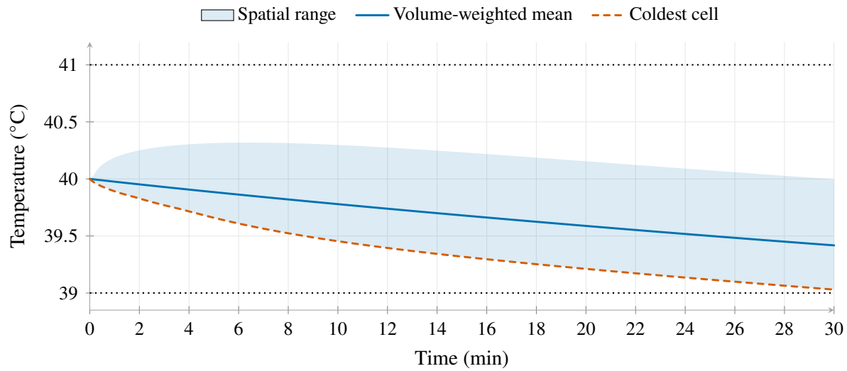
Figure 2. Matrix-exponential cell temperatures under the selected policy. The shaded range covers the coldest cell and the hottest cell outside the inlet jet zone; the mean alone would hide cold and hot locations.
