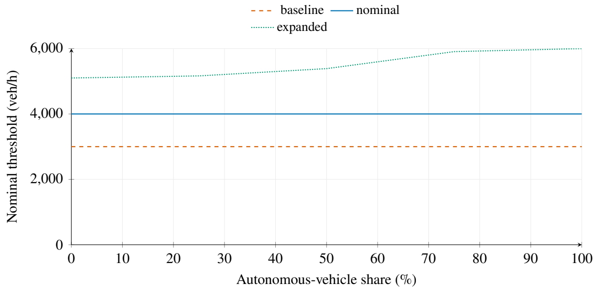
Figure 4. Headway improvement matters only when an exit-related cut is limiting. A flat curve means that the service/compatibility bottleneck remains.
