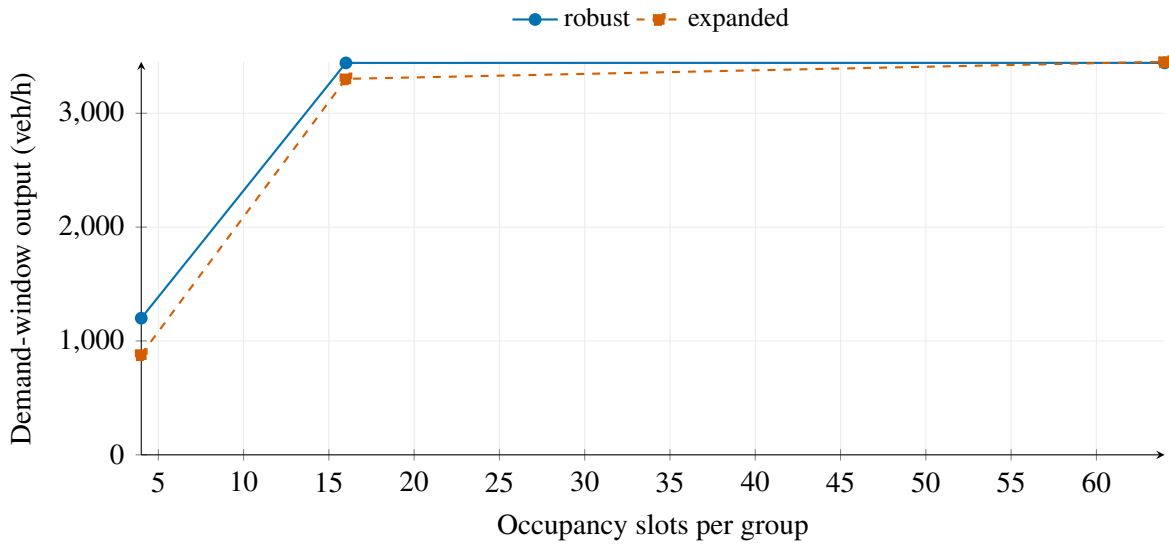
Figure 3. Nominal heavy-demand output with finite occupancy. These are transient observed rates, distinct from the compatible-flow arrival thresholds.
