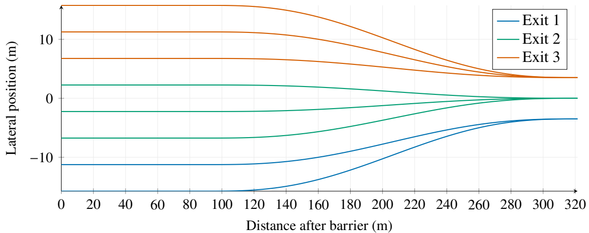
Figure 1. Order-preserving centerline paths for the selected nominal design. Curves within one group merge at its assigned exit. Release spacing is a separate control requirement.
