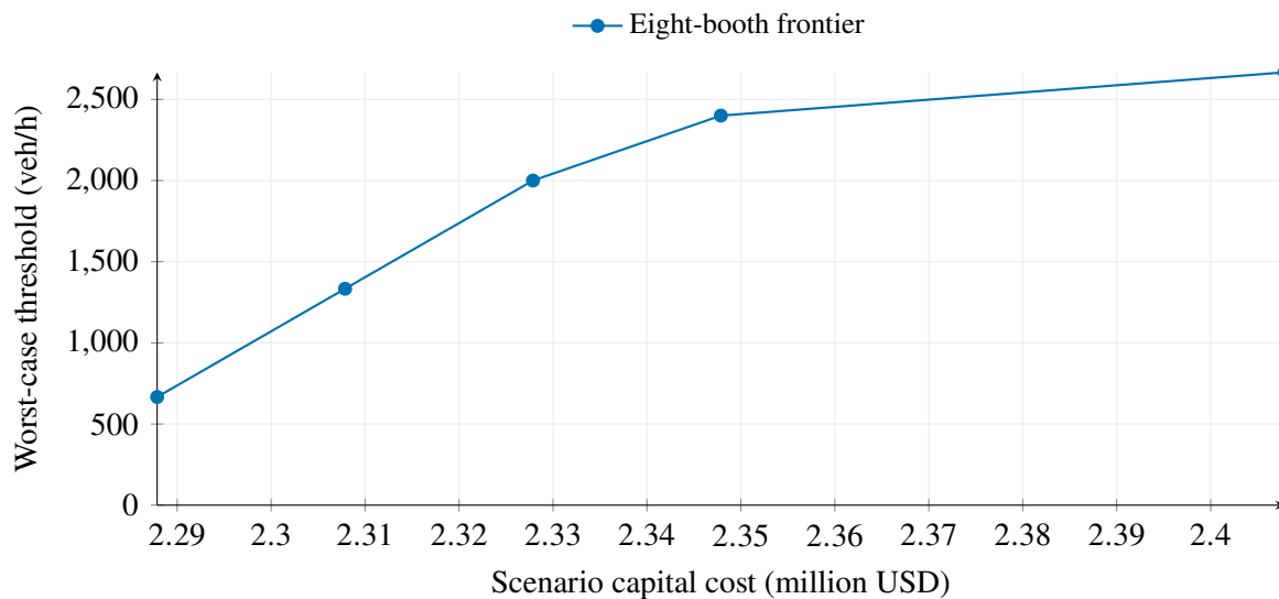
Figure 2. Nondominated cost/capacity points within the enumerated eight-booth family. Different land prices or admissible routing rules can change this frontier.
