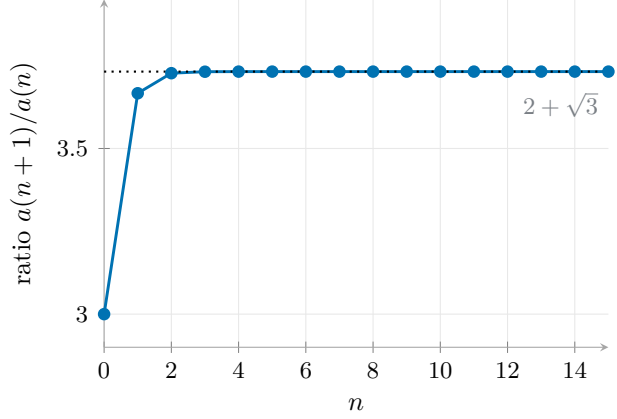
Figure 1. Consecutive-term ratios and the proved limit 2 + \sqrt{3} .
