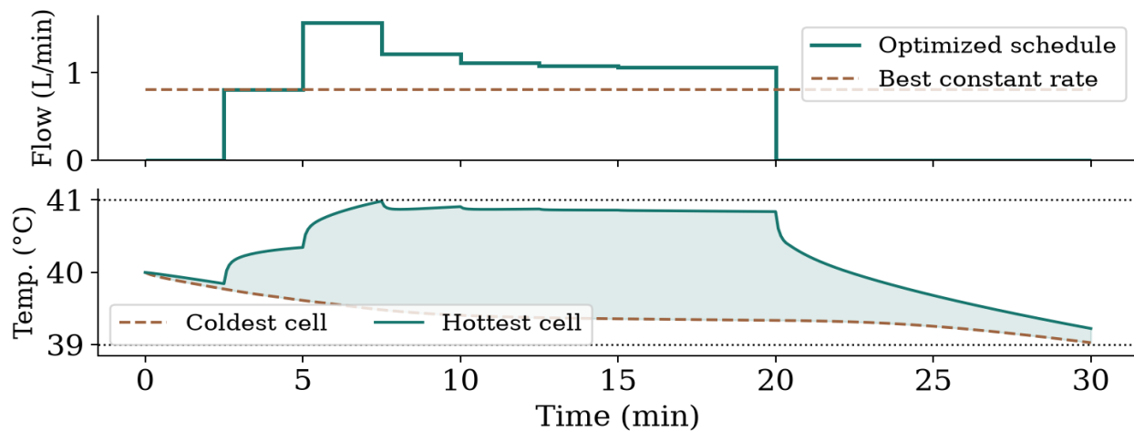
Figure 6. Best 12-segment schedule against the best constant rate (top) and the range of cell temperatures (bottom); dotted lines mark the limits.
