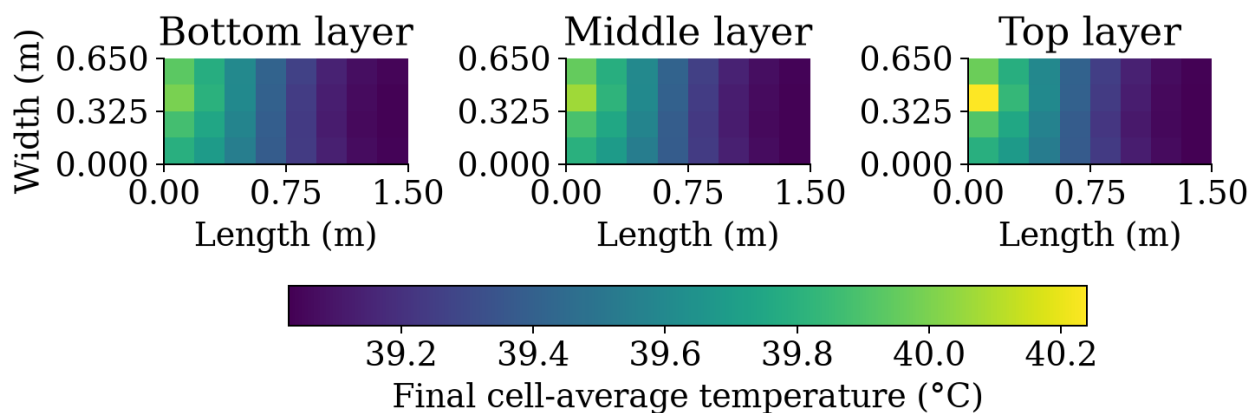
Figure 4. Final temperatures in the three horizontal cell layers. All layers use one color scale; the top layer contains the prescribed inlet-to-overflow stream. Geometry is in metres, and values are cell averages.
