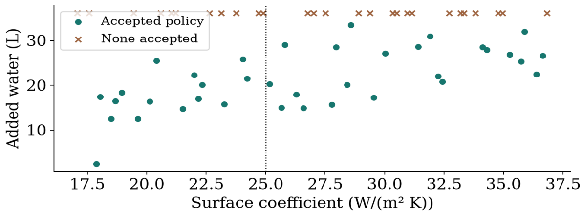
Figure 8. Required water against the surface coefficient for each Sobol draw. Crosses at the top mark draws with no accepted policy; the vertical line is the baseline.
