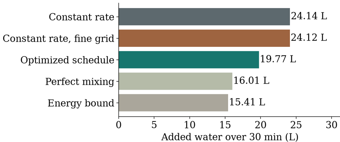
Figure 7. Water-use comparison under the same lower limit. The energy bound is conditional on the network assumptions; the feasible spatial result remains above it.
