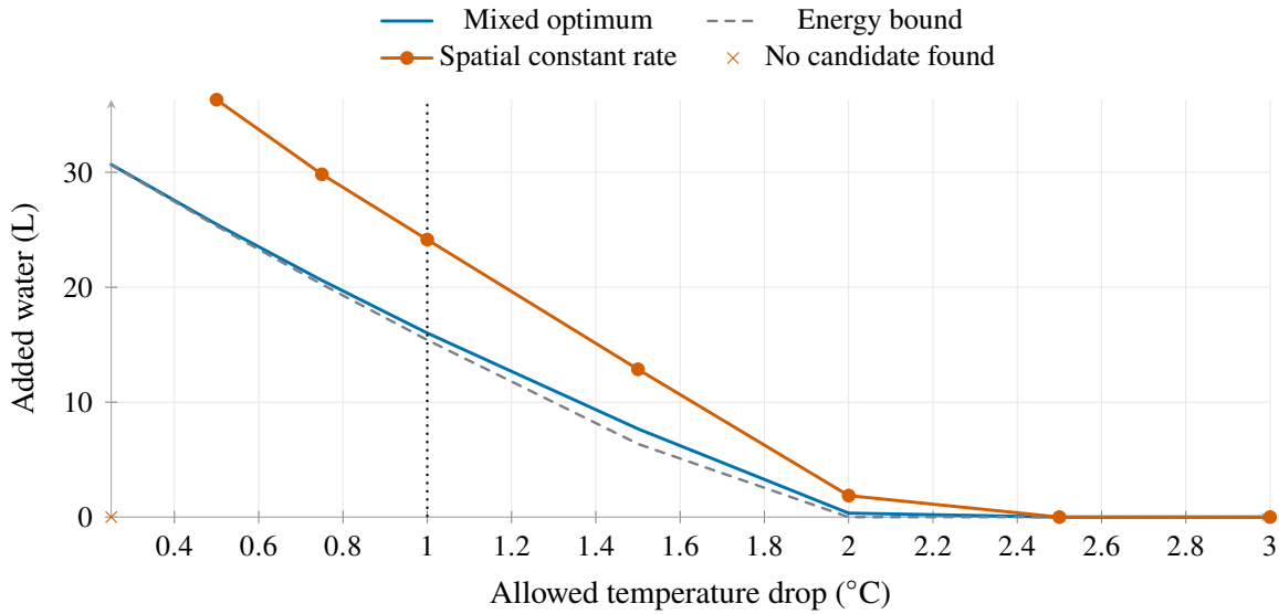
Figure 5. Water use versus temperature tolerance. Crosses denote unsuccessful searches, not zero water demand; the dotted line marks the baseline.
