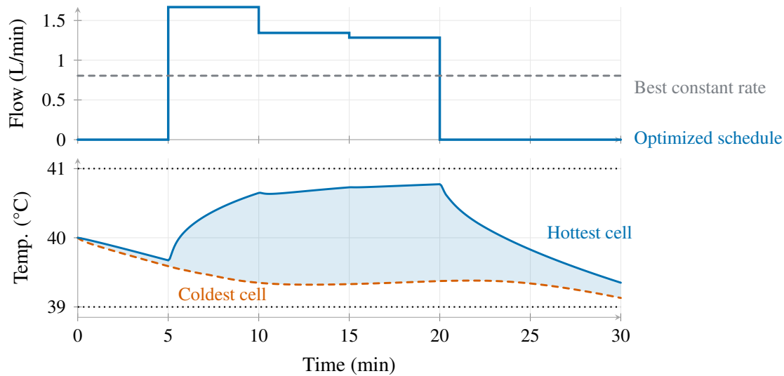
Figure 4. Selected buffered 6-segment schedule against the best constant rate (top) and the range of cell temperatures outside the inlet jet zone (bottom); dotted lines mark the limits.
