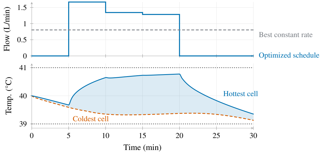
Figure 3. Selected buffered 6-segment schedule against the best constant rate (top) and the range of cell temperatures outside the inlet jet zone (bottom); dotted lines mark the limits.
