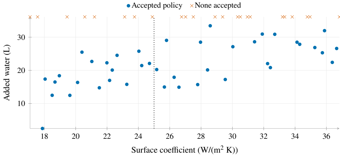
Figure 5. Required water against the surface coefficient for each Sobol draw. Crosses at the top mark draws with no accepted policy; the vertical line is the baseline.
