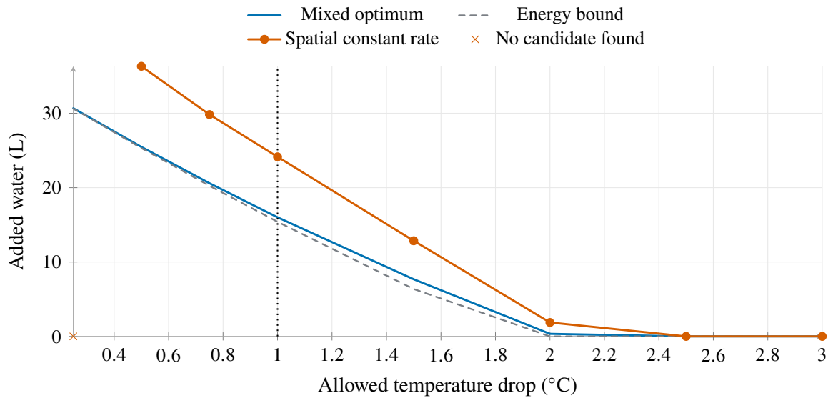
Figure 4. Water use versus temperature tolerance. Crosses denote unsuccessful searches, not zero water demand; the dotted line marks the baseline.
