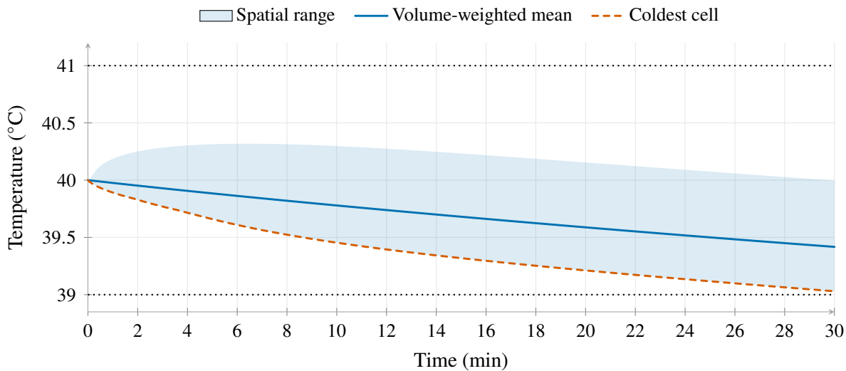
Figure 3. Matrix-exponential cell temperatures under the selected policy. The shaded range covers the coldest cell and the hottest cell outside the inlet jet zone; the mean alone would hide cold and hot locations.
