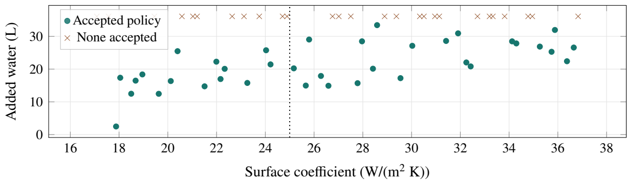
Figure 7. Required water against the surface coefficient for each Sobol draw. Crosses at the top mark draws with no accepted policy; the vertical line is the baseline.
