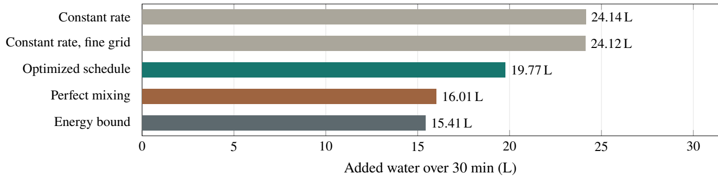
Figure 6. Water-use comparison under the same lower limit. The energy bound is conditional on the network assumptions; the feasible spatial result remains above it.
