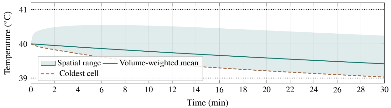
Figure 3. Matrix-exponential cell temperatures under the selected policy. The shaded range includes all cells; the mean alone would hide cold and hot locations.
