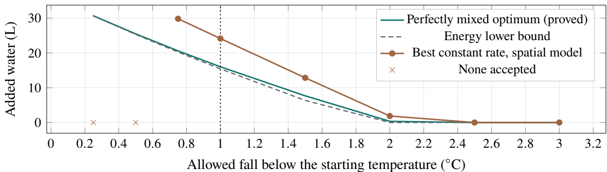
Figure 5. Added water against the allowed temperature fall. The mixed optimum and energy bound are closed forms; markers on the brown curve are searched constant-rate policies, and the dotted line is the baseline.
