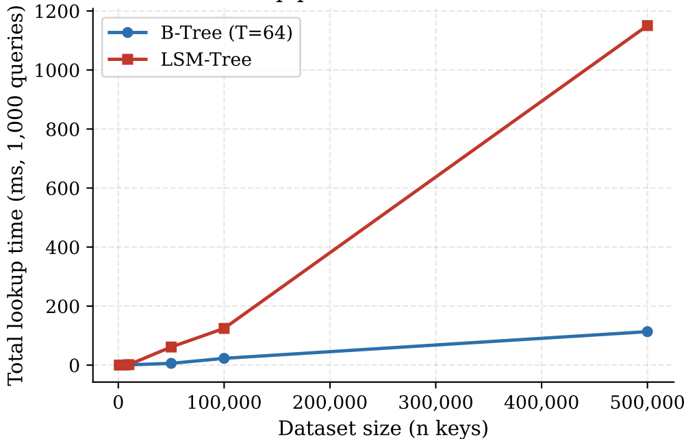
Point lookup performance vs. dataset size
