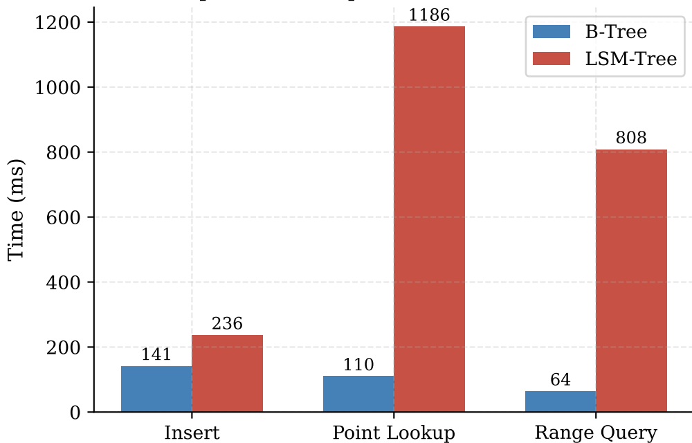
Operation comparison at n = 500,000
