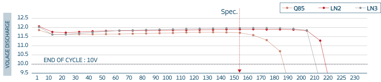
DOD 50% CYCLE
