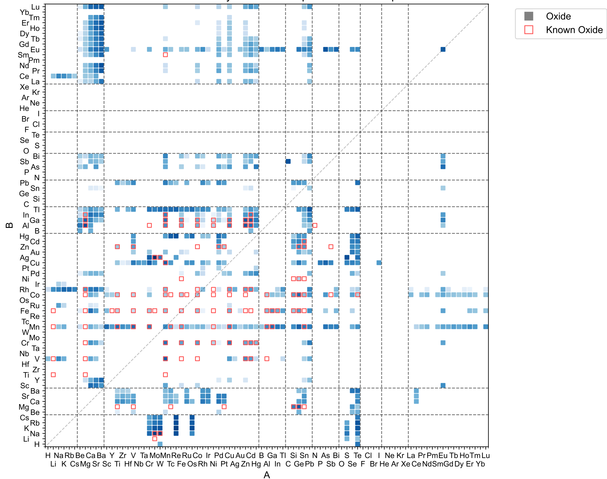
Known and Chemically Valid Oxide Spinel Chemical Space
