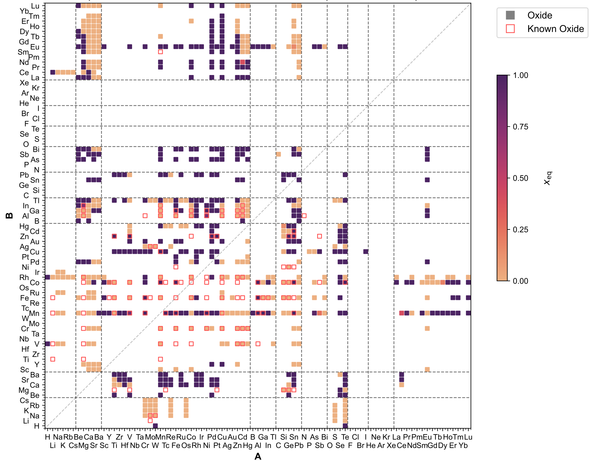
Equilibrium Cation Inversion Parameter of Oxide Spinel Chemical Space
