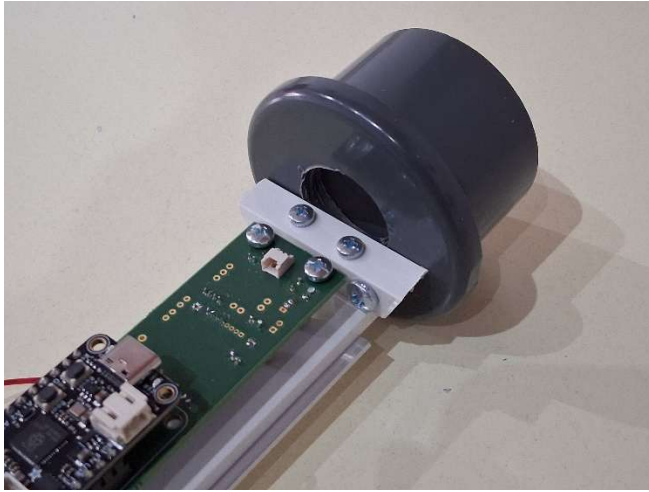
Figure 5: using PVC and ALU bars mounted on endcap (B)
