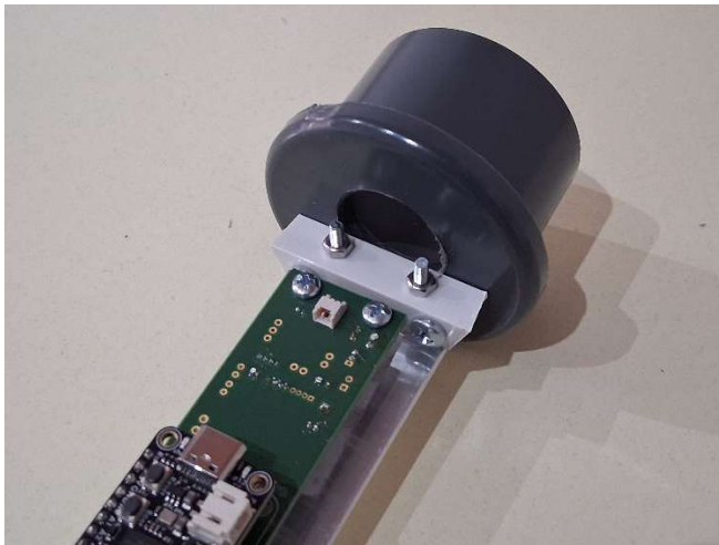
Figure 6: Using only ALU bar mounted on endcap (B)
