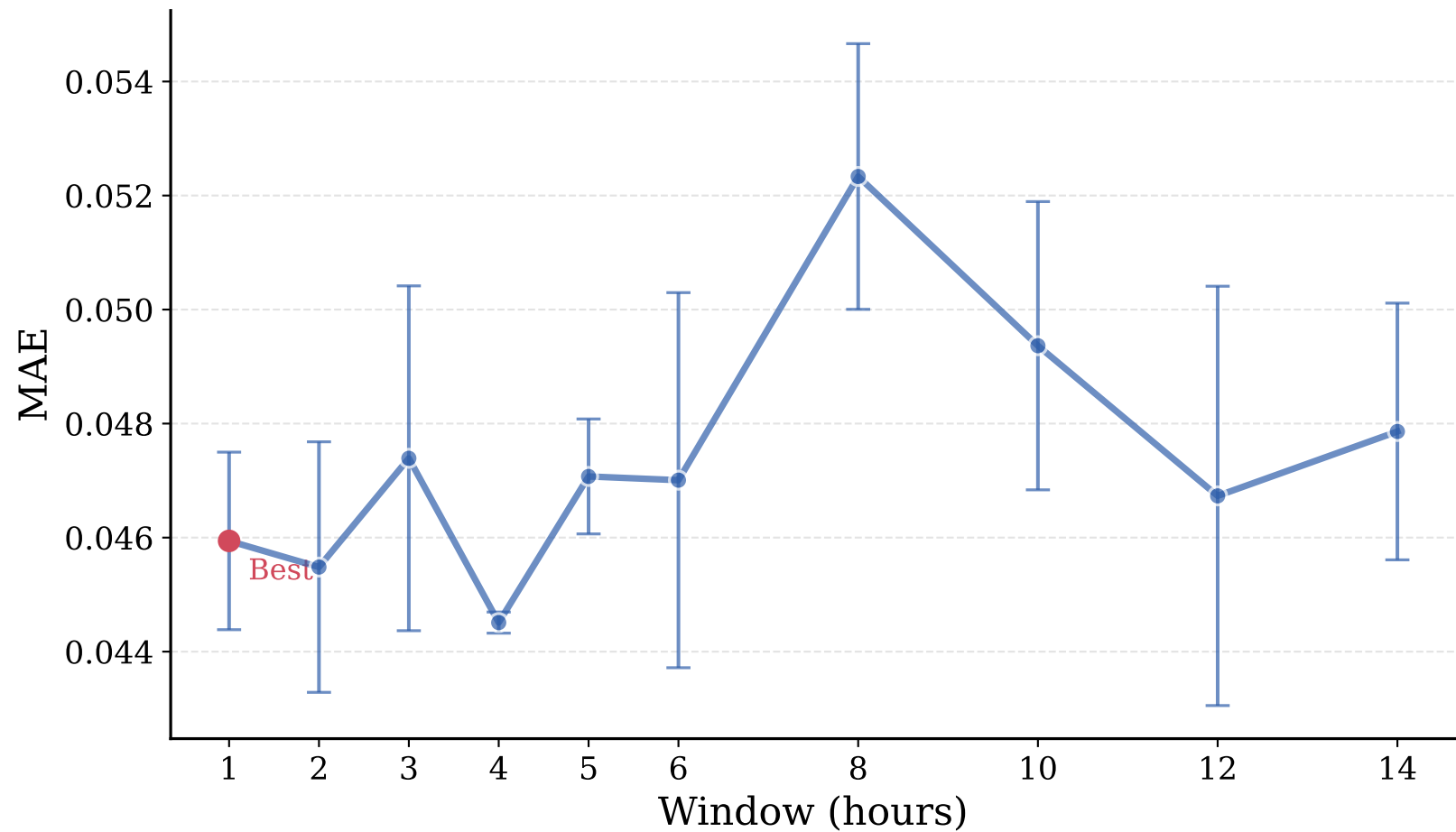
Window Length vs MAE (mean \pm std)
