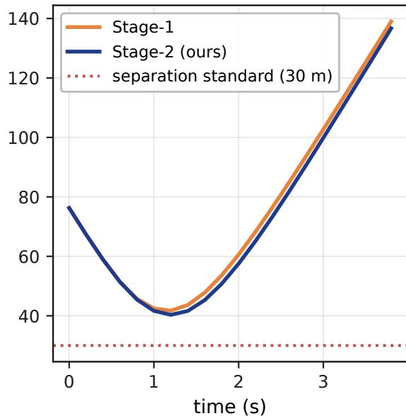
(b) Separation profile
