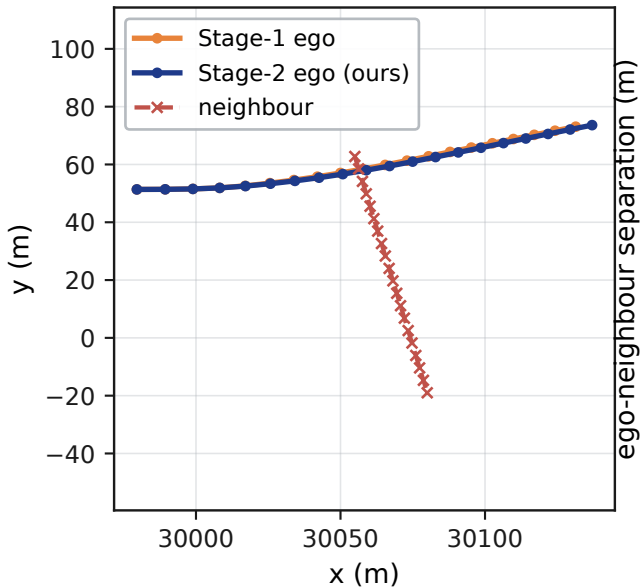
(a) Closed-loop trajectories
