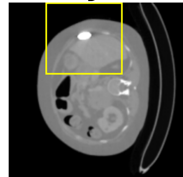
Polyner
