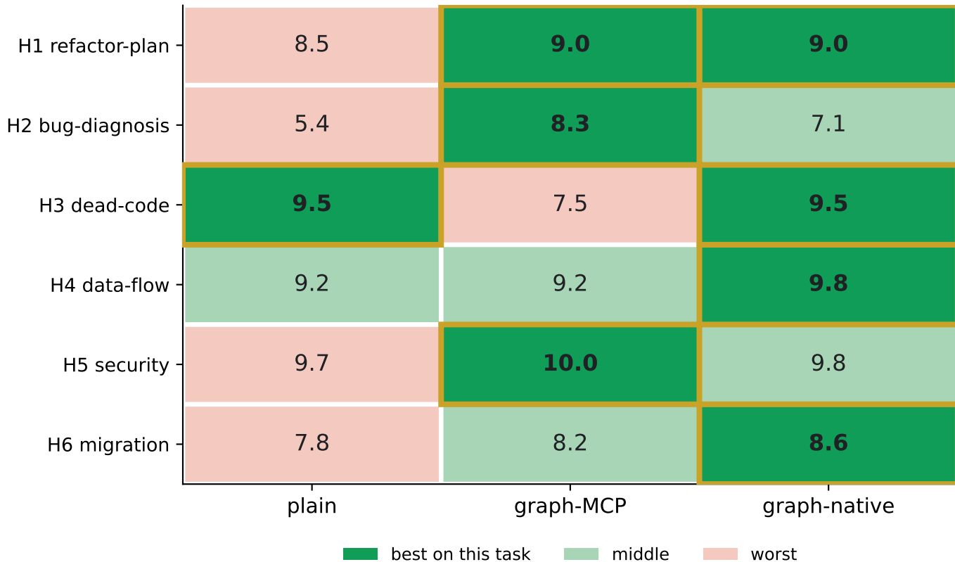
Per-task quality — green = best for that task, gold box = winner (cell number is the 0-10 judge score)
