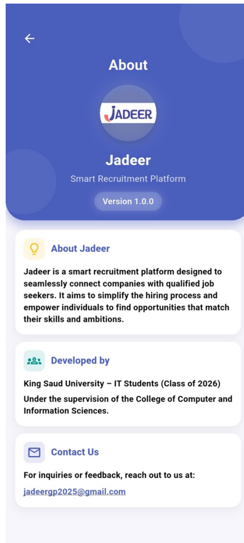
Figure 33: About Page.
