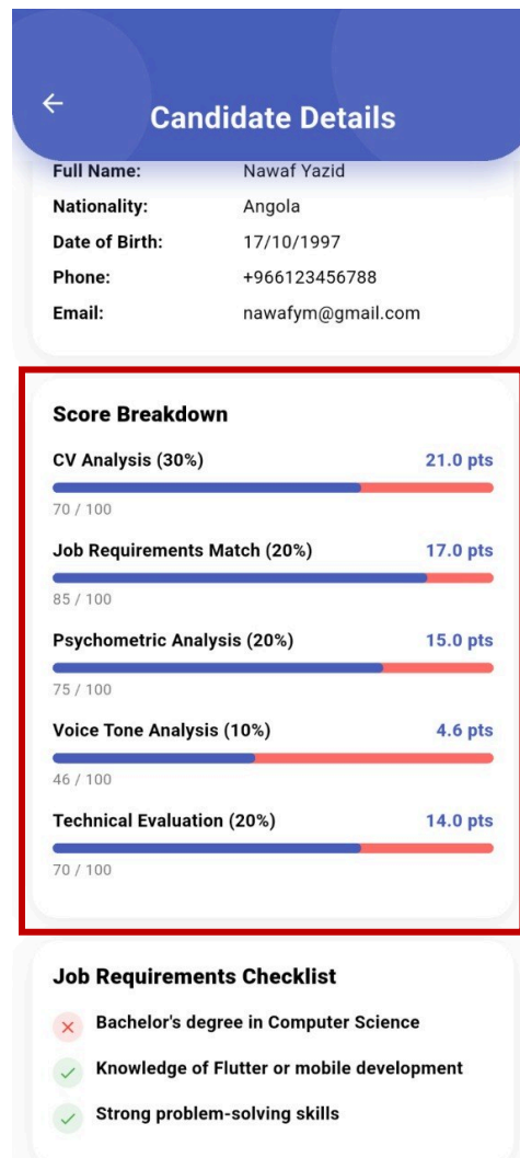
Figure 109: Score breakdown.
