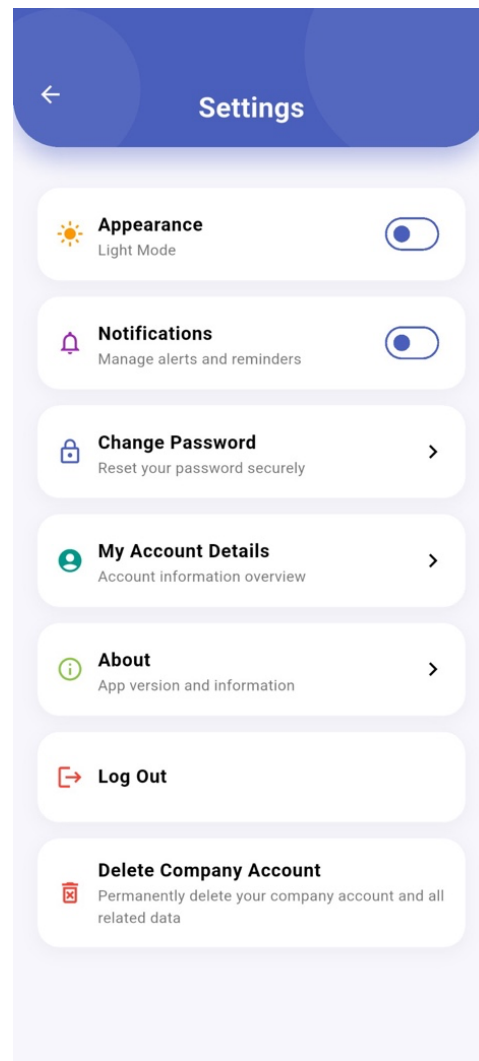
Figure 22: Settings Page.
