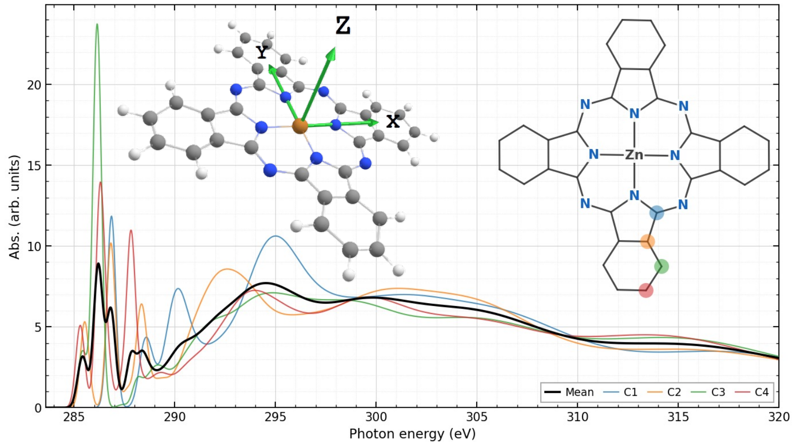
Site-resolved X-ray spectra
