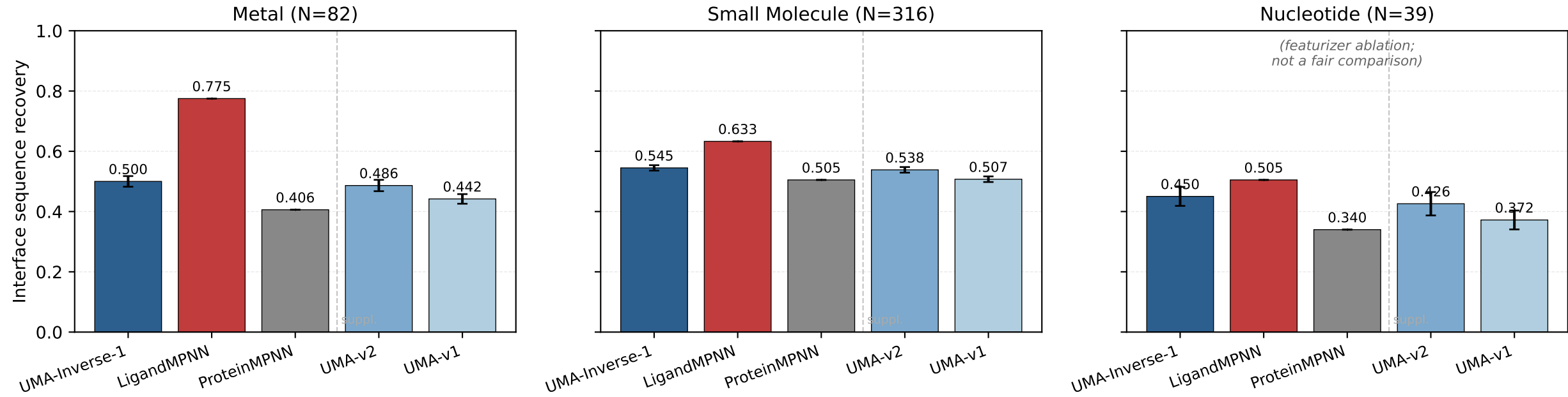
Interface sequence recovery, LigandMPNN-paper protocol (10 designs/PDB, T=0.1, random decoding, 5Å sidechain cutoff) — UMA-v2/v1 bars are supplemental
