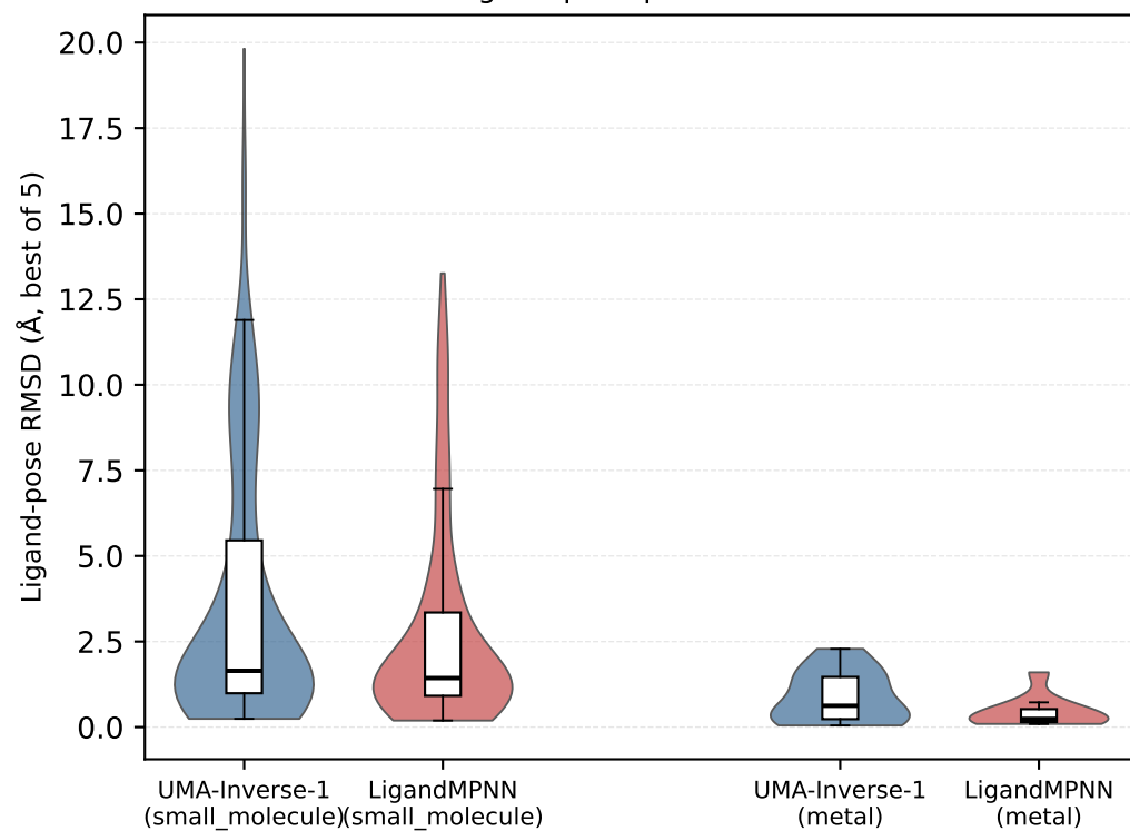
Ligand-pose preservation
