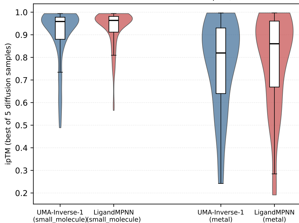
Ligand-pose preservation
