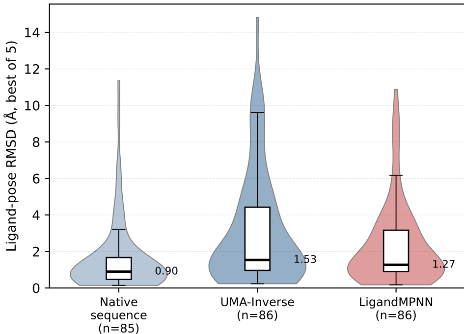
Cofold ligand-pose RMSD (LigandMPNN vs UMA: paired p=0.003 )
