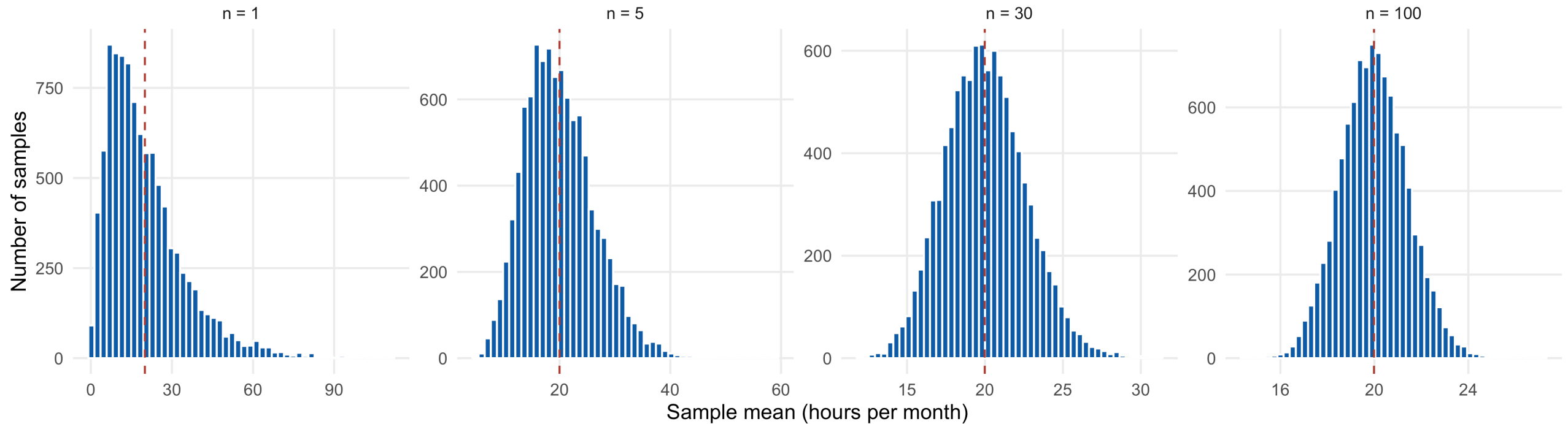
Distribution of 10,000 sample means for different sample sizes n (skewed population)
