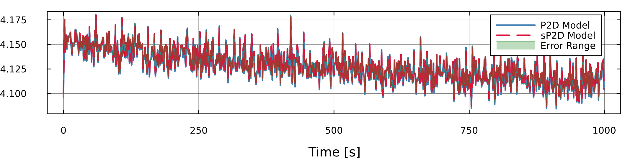
Figure 2: Internal State Evolution Mechanism Concentration gradients and overpotential dynamics drive electrochemical
