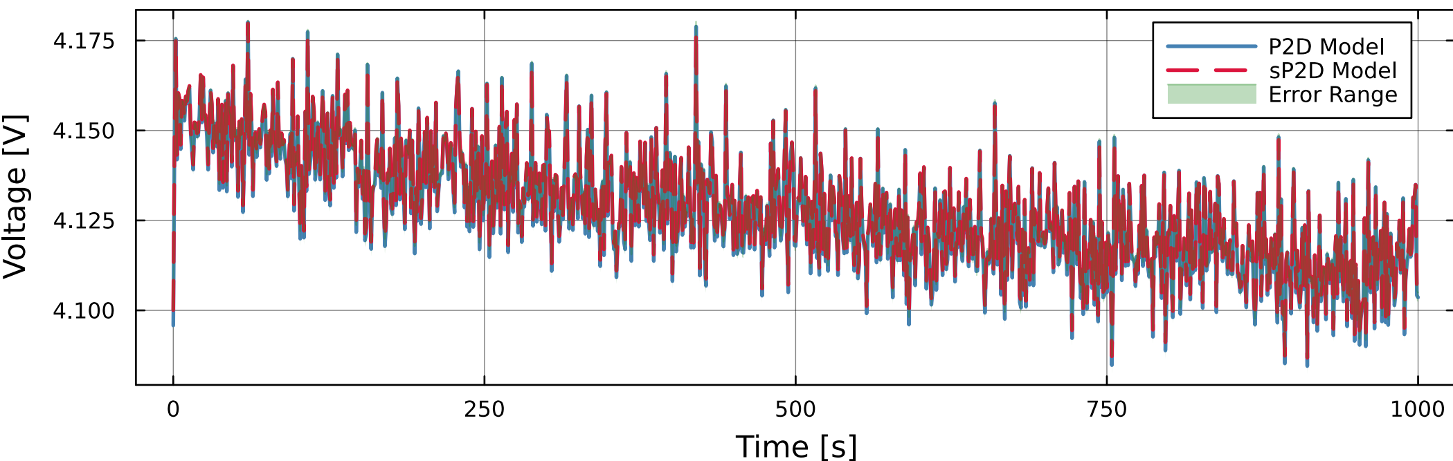
(b) Cell Voltage Response
