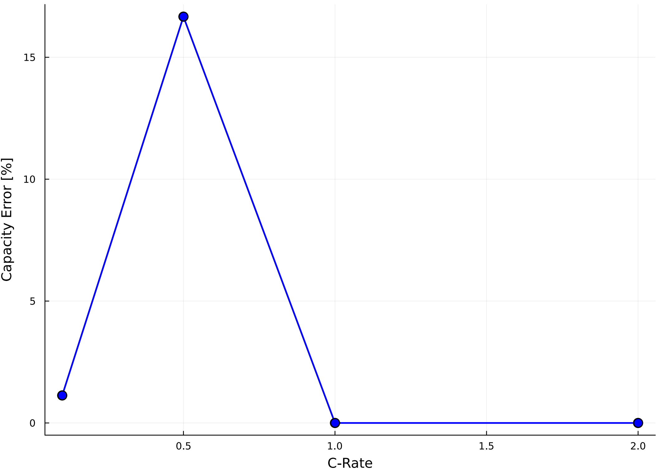
Capacity Error vs C-Rate
