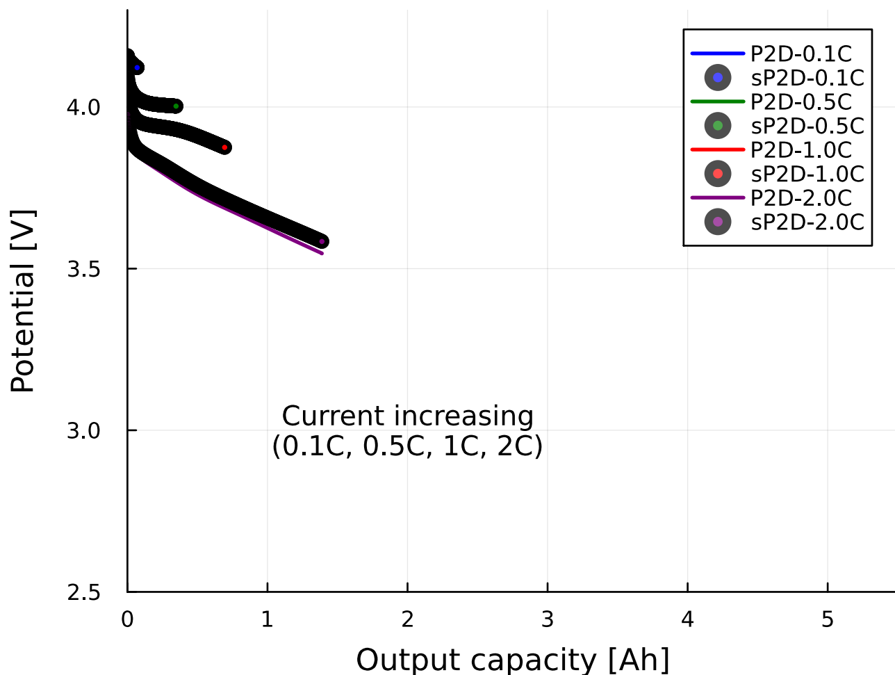
Capacity Difference between P2D and sP2D
