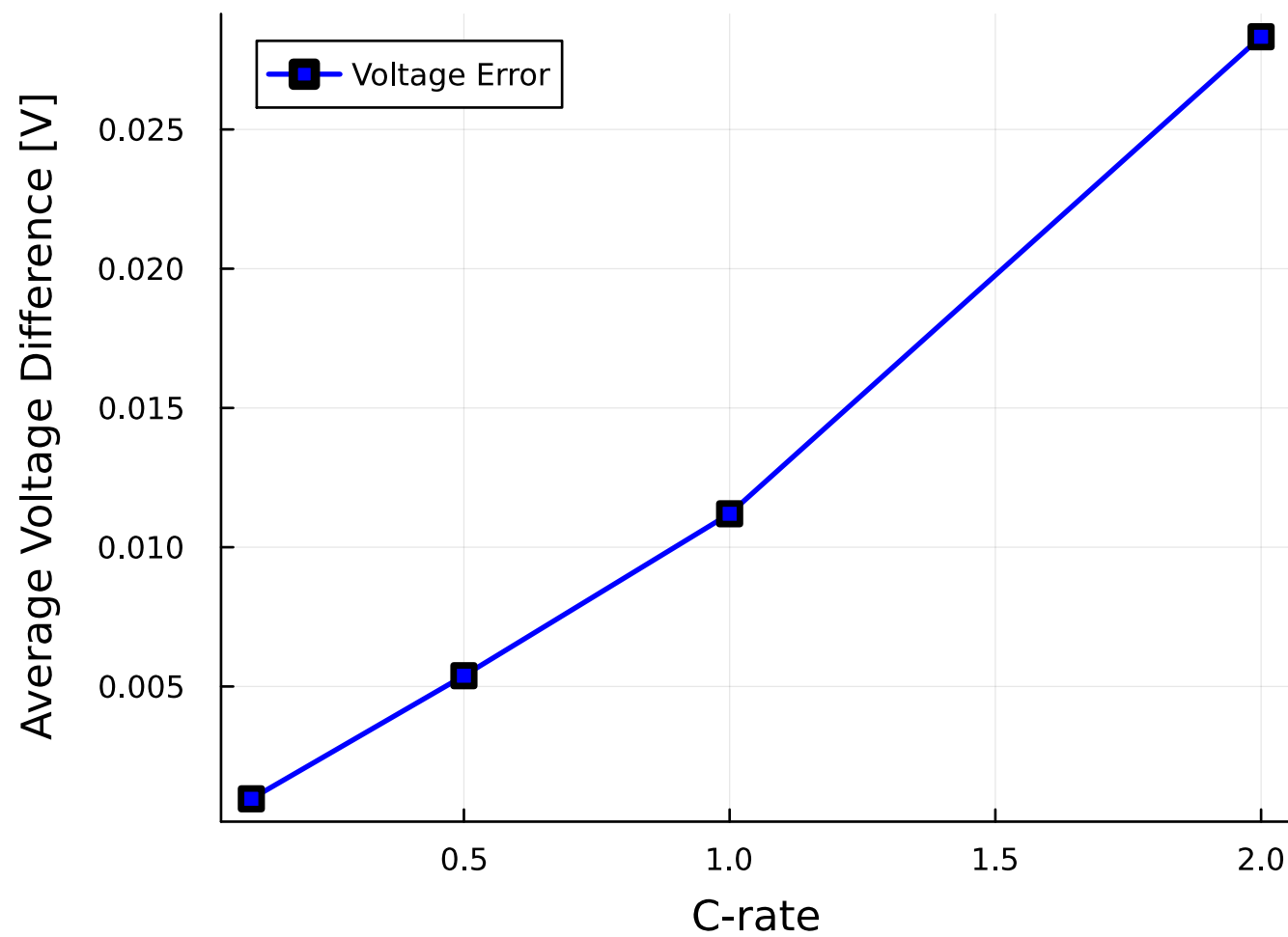
Voltage Difference between P2D and sP2D
