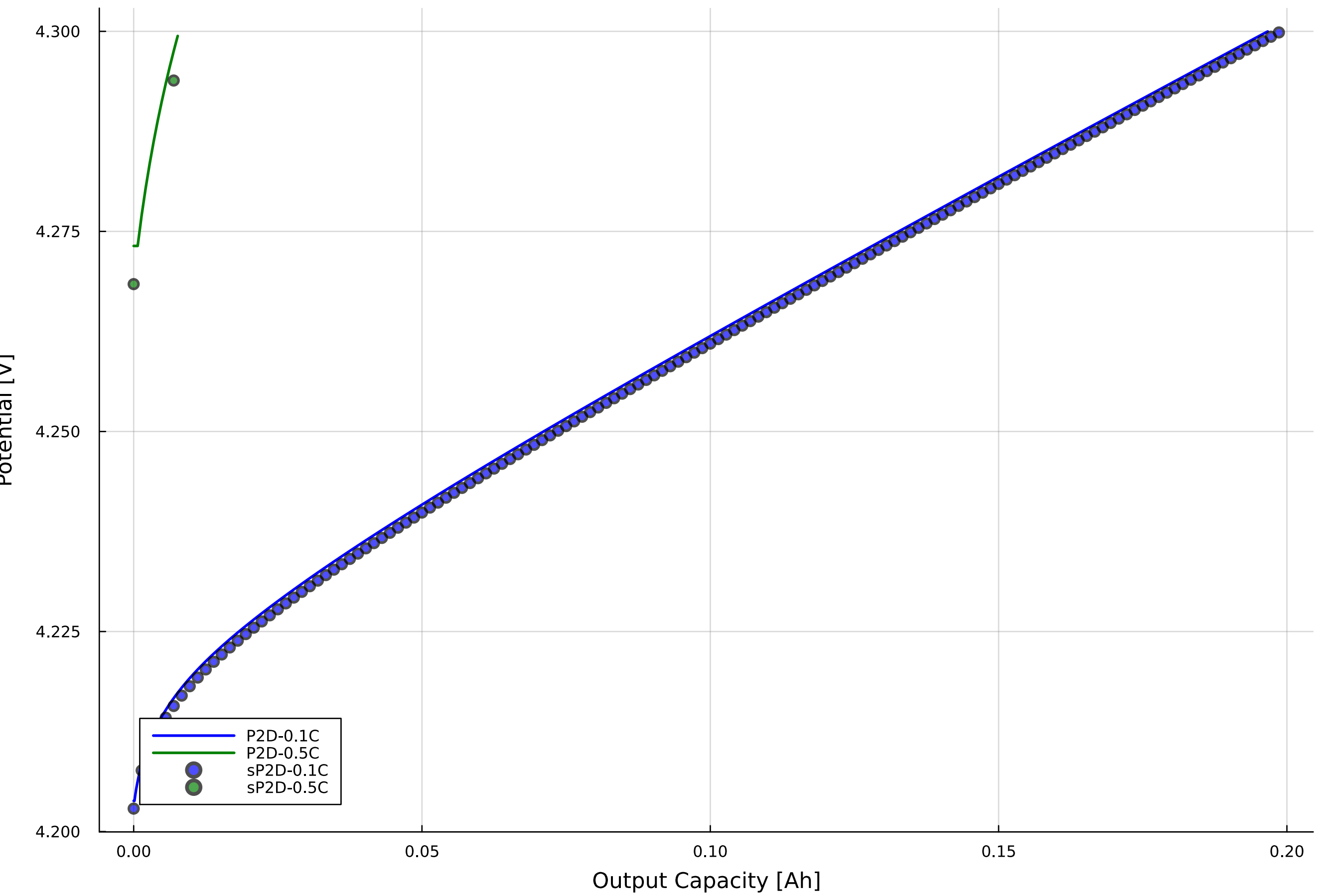
Discharge Performance Comparison: P2D vs sP2D at Different C-rates
