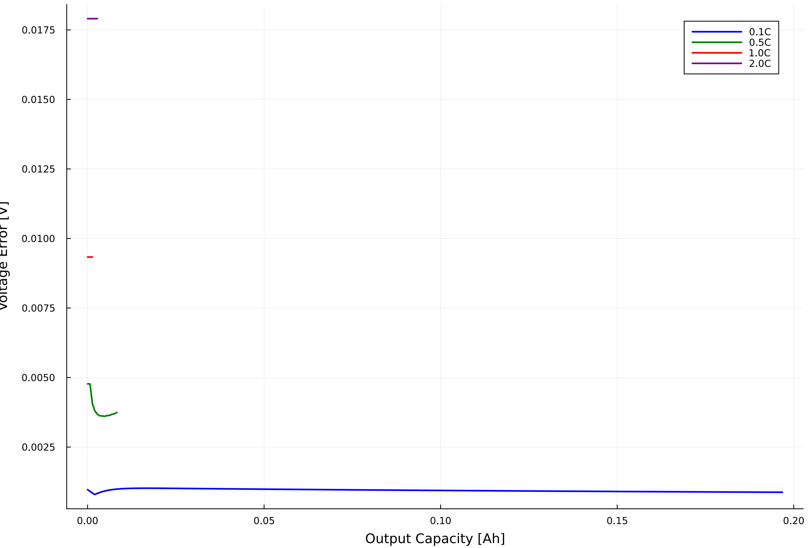
Voltage Error: |sP2D - P2D| at Different C-rates
