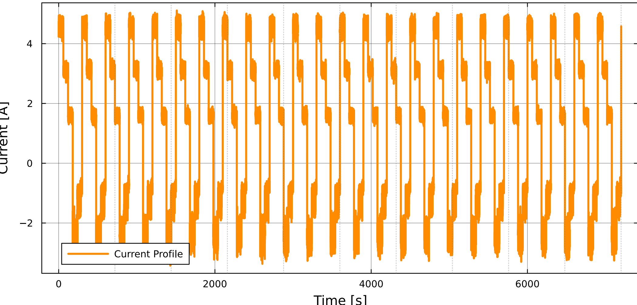
Fast Charge-Discharge Current Profile
