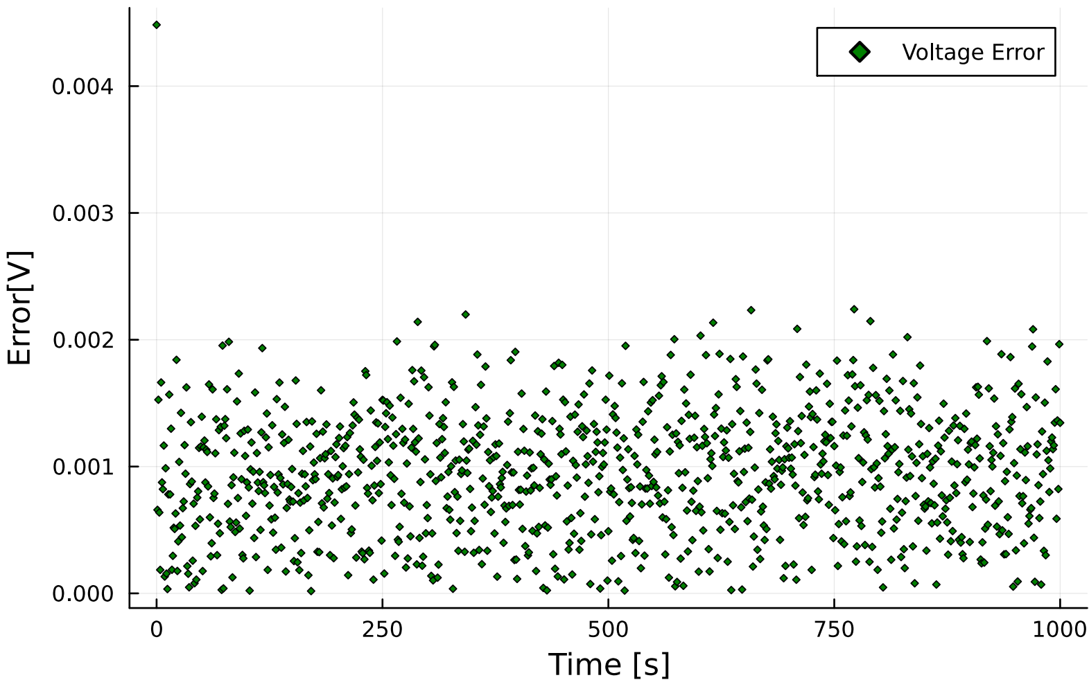
Model Voltage Error Comparison (P2D vs sP2D)
