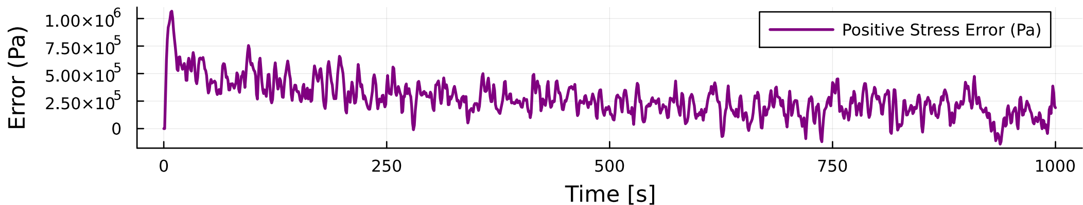
Positive Stress Error Comparison (P2D vs sP2D)
