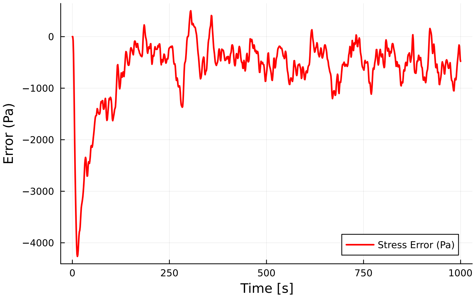
Stress Error Comparison (P2D vs sP2D)
