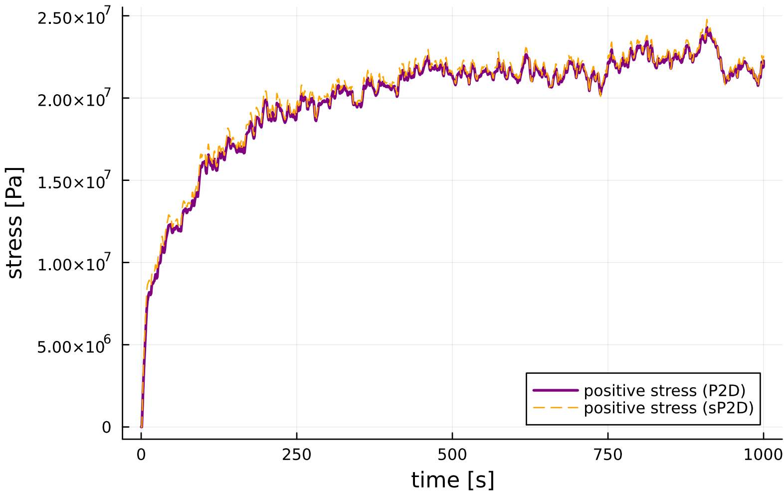
positive stress comparison (P2D vs sP2D)
