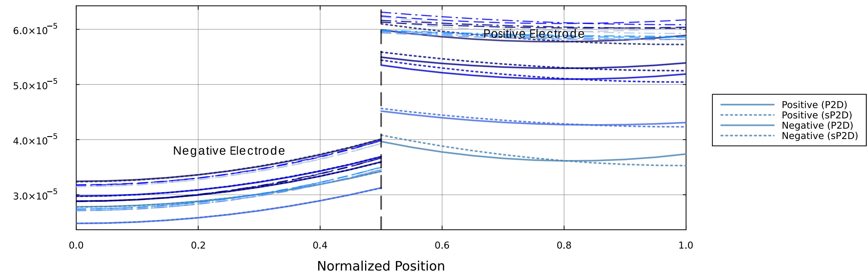
High Frequency Pulse Current Profile
