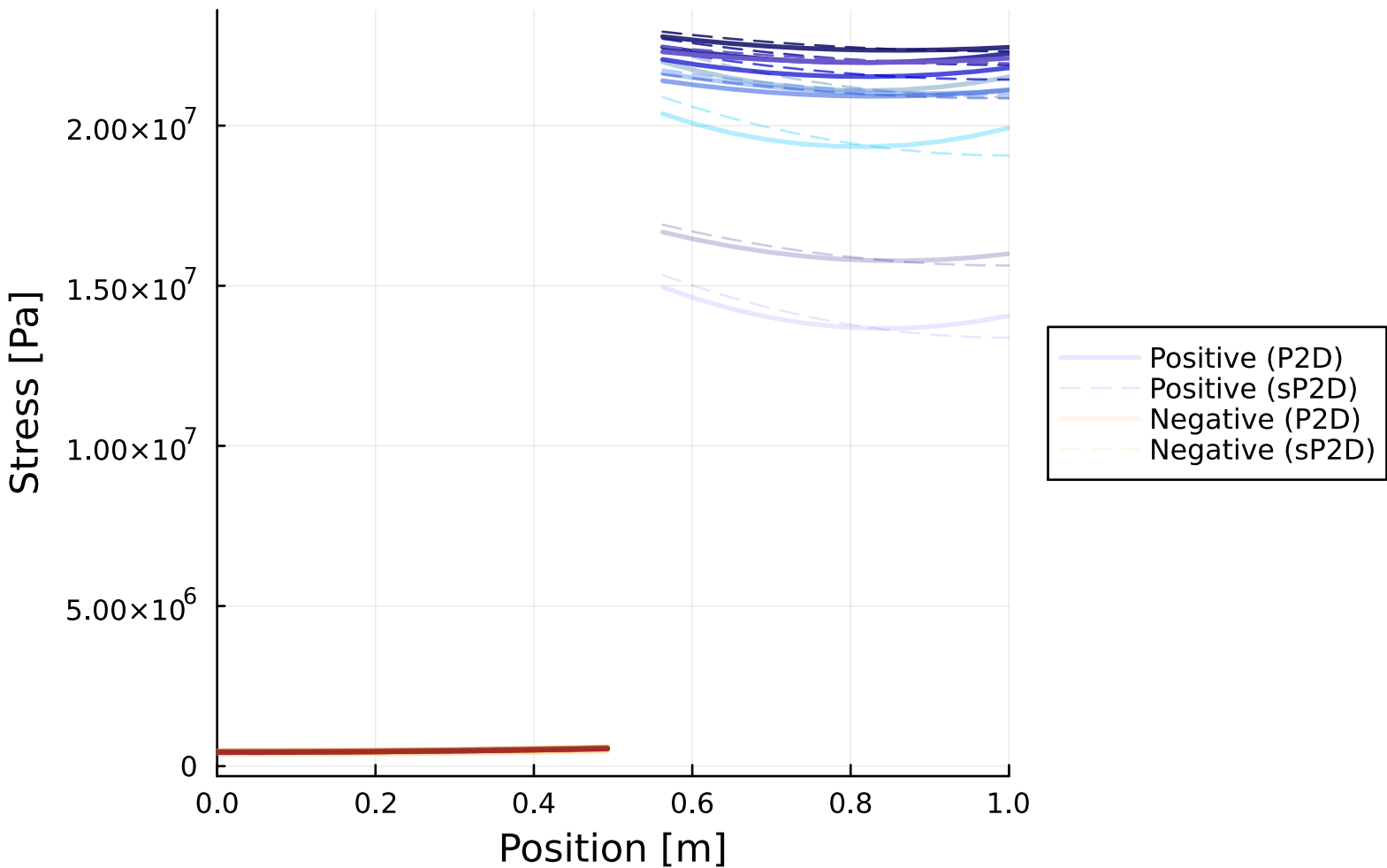
The Stress Distribution (P2D & sP2D) - High Frequency Pulse
