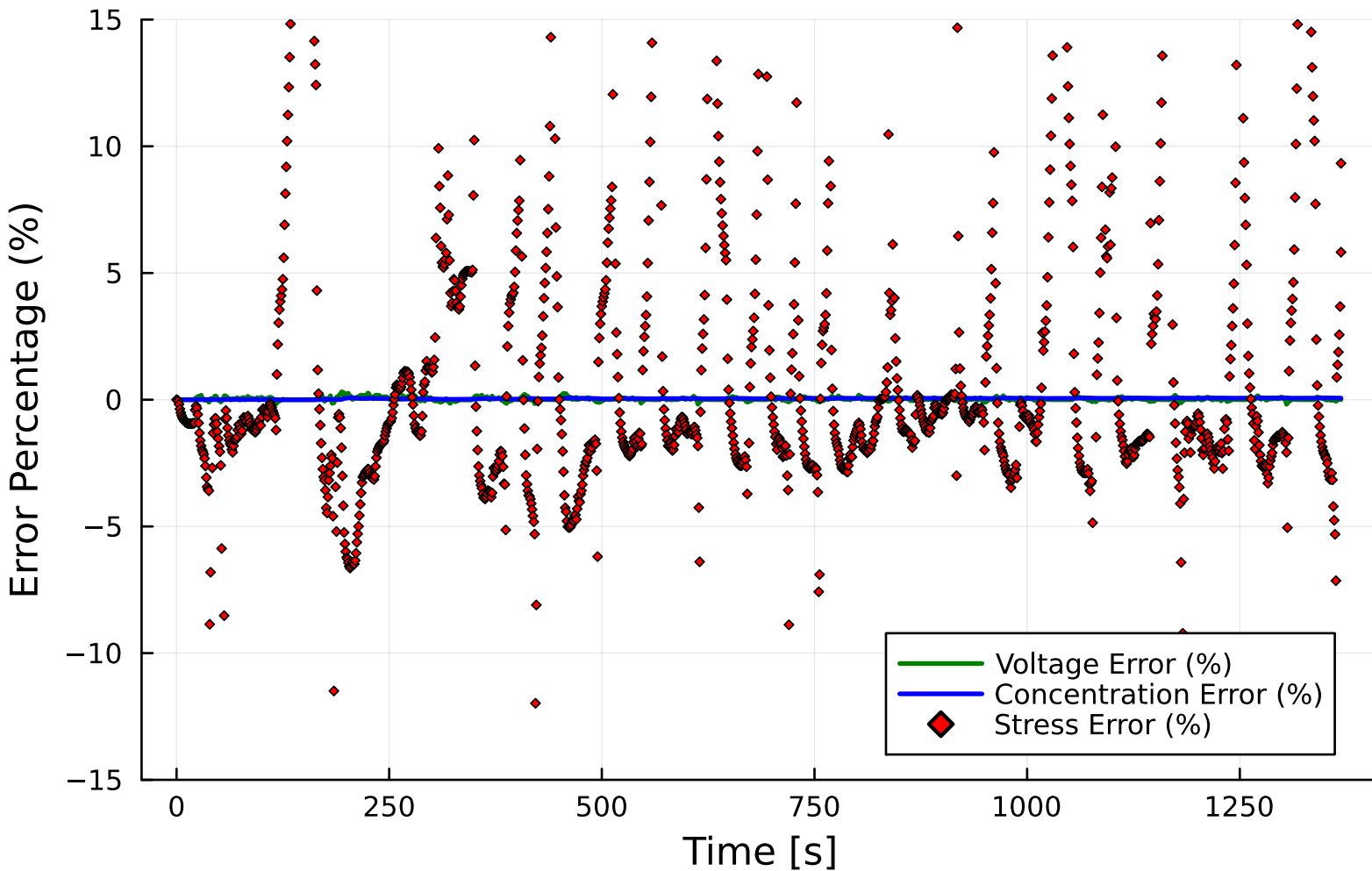
Model Error Comparison (P2D vs sP2D)
