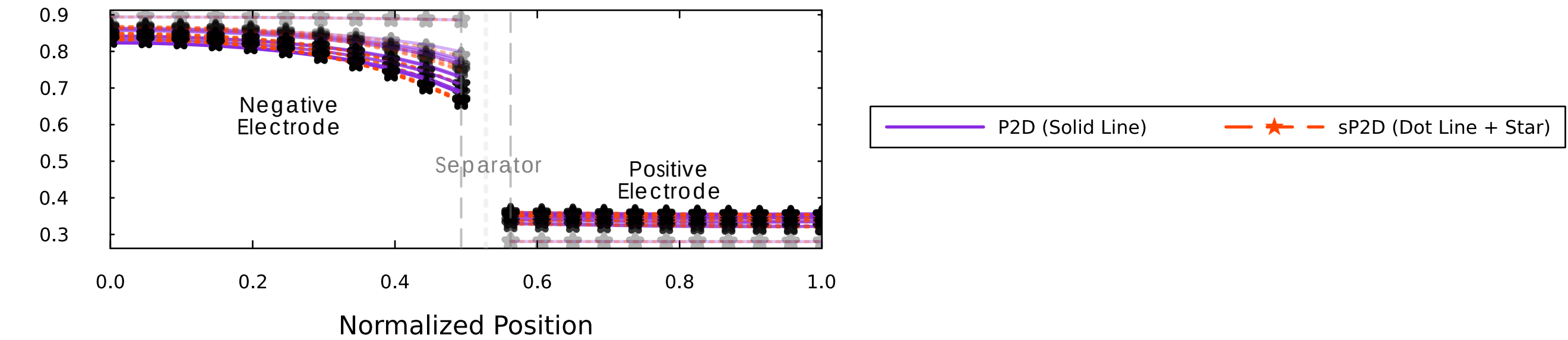
Electrode Stress Distribution - Normalized
