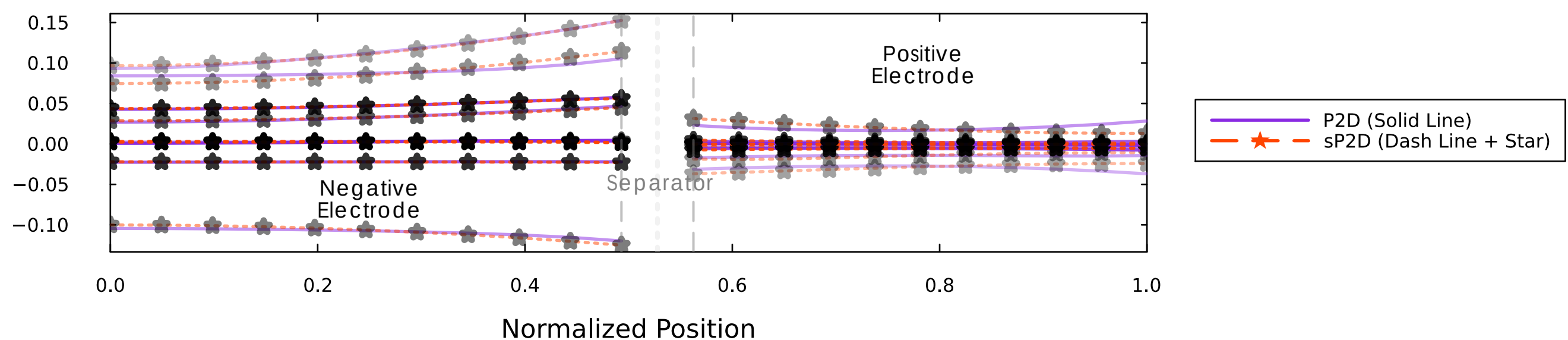
Electrode Potential Distribution
