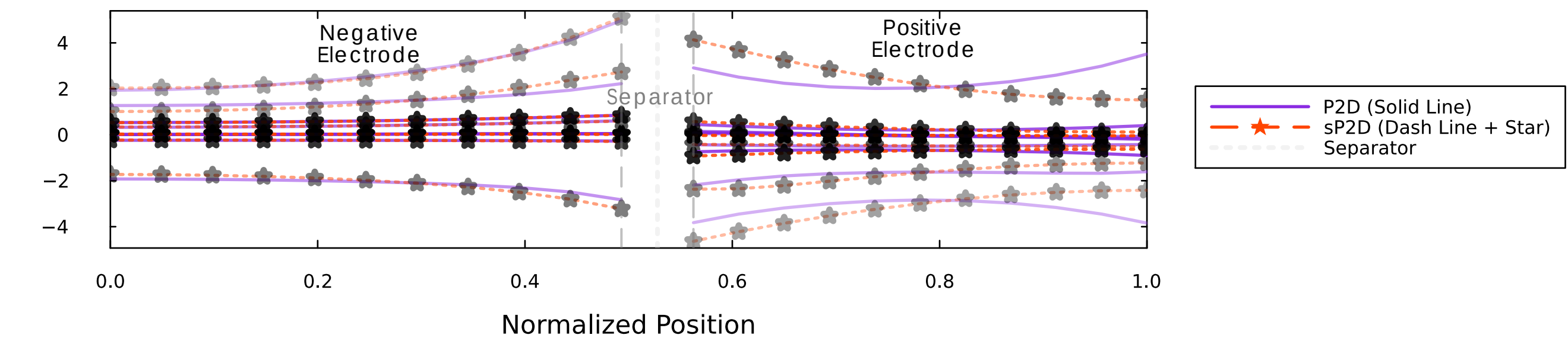
Electrode Overpotential Distribution
