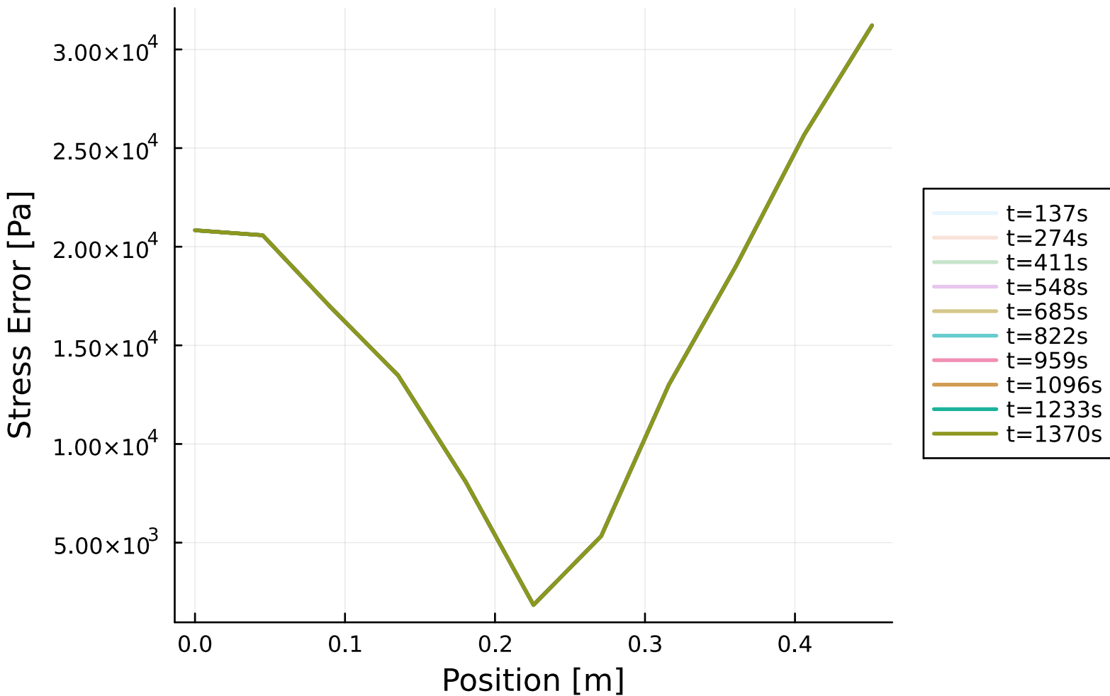
Spatial Stress Error (sP2D vs P2D) - UDDS
