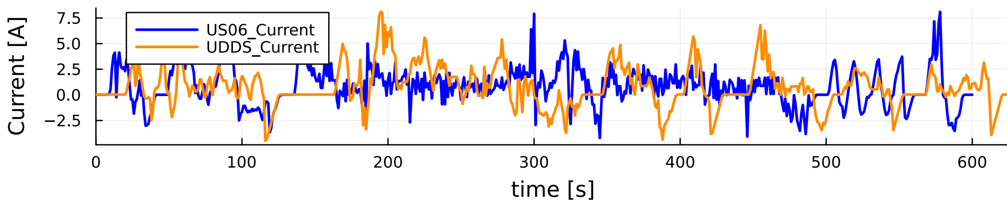
UDDS and US06 Current Profile
