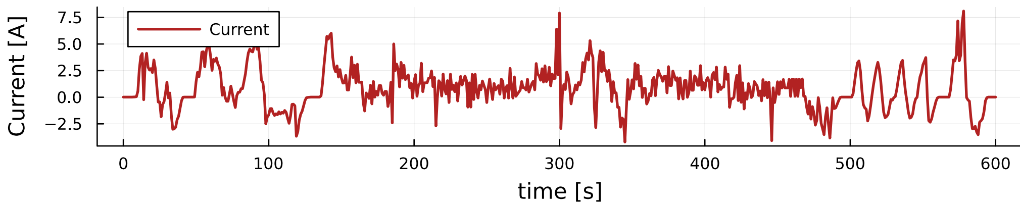
US06 Current Profile
