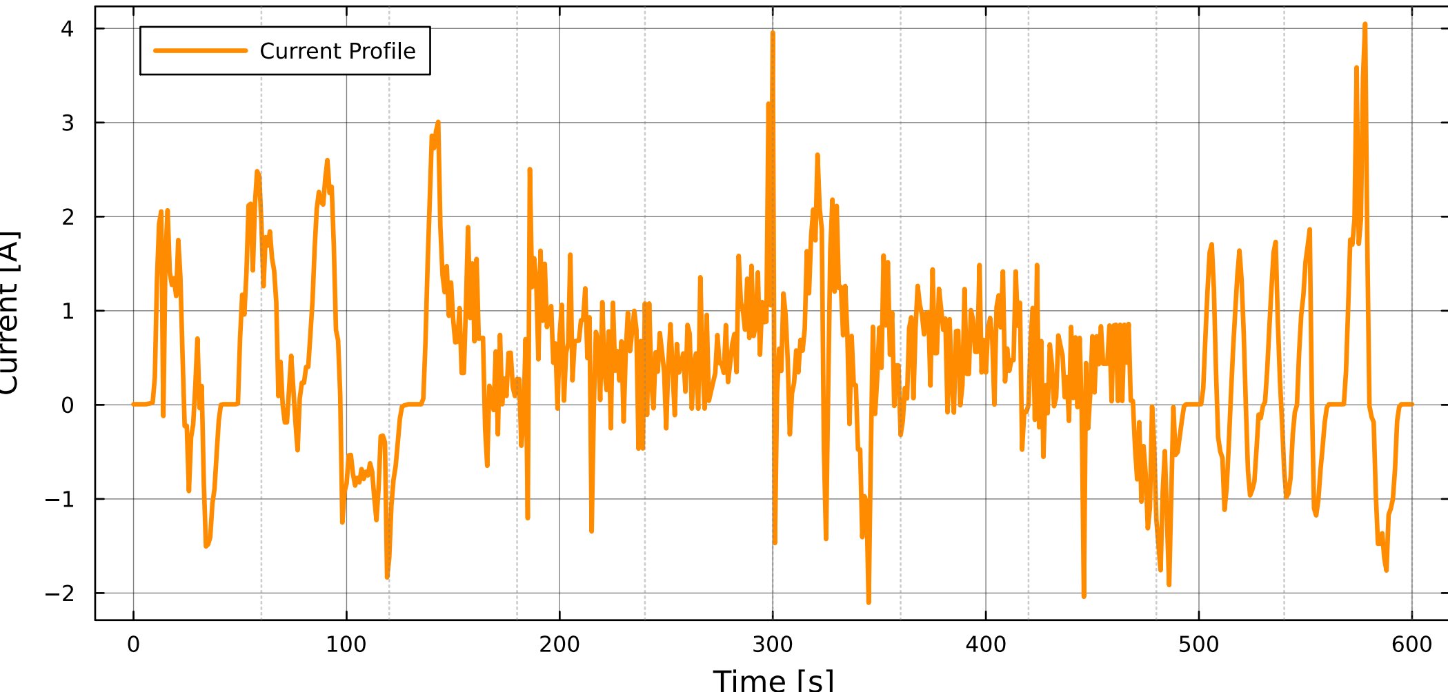
US06 Current Profile
