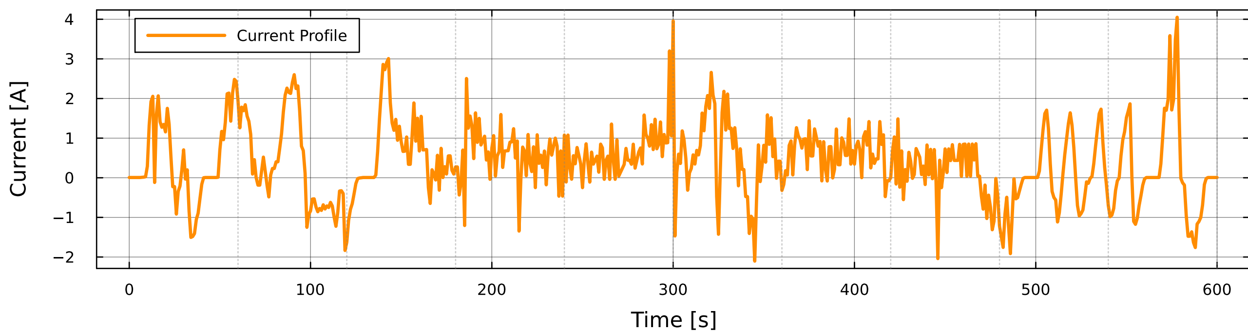
US06 Current Profile
