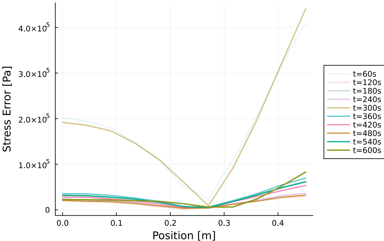
Spatial Stress Error (sP2D vs P2D) - US06
