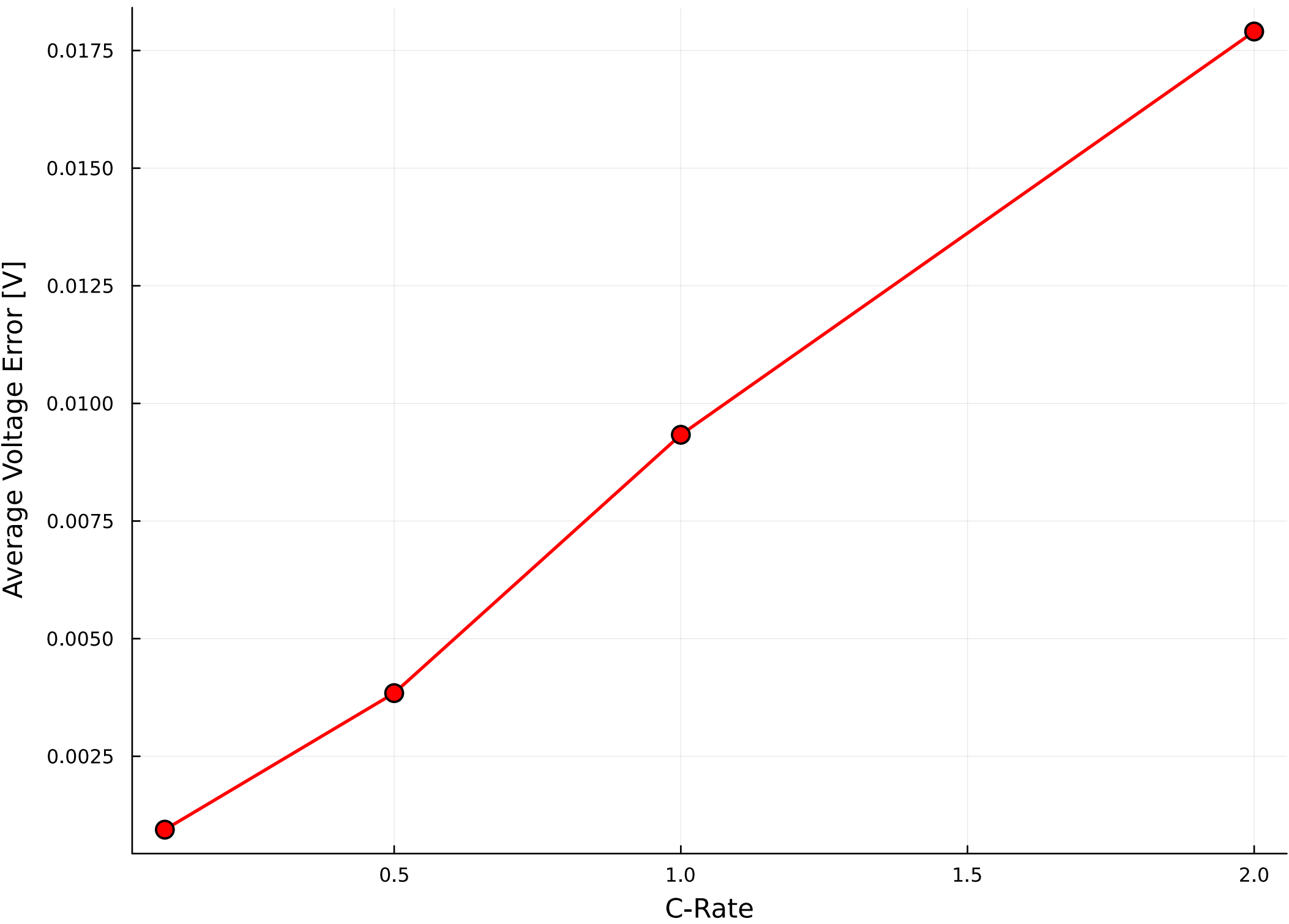
Average Voltage Error vs C-Rate
